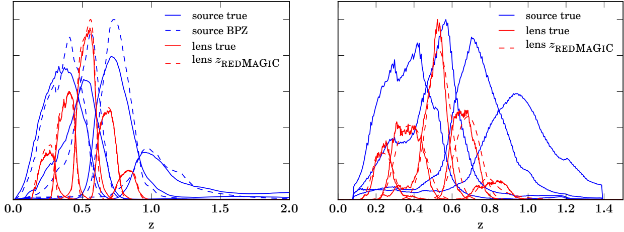
Figure 1. Redshift distributions for the galaxy samples used. Red and blue indicate the REDMAGIC ( lens ) galaxies and the weak lensing source galaxies respectively. Solid and dashed lines indicate the true distributions and those estimated from photometric redshifts respectively. Left panel: BCC, right panel: MICE. As discussed in Section 4.2, we do not have BPZ photo- z estimates for the weak lensing source sample in MICE and by construction the true source redshift distributions match the BPZ estimates for the real data, apart from above z = 1.4 , the maximum redshift of the MICE galaxies. For visual clarity, the lens and source redshift distributions have arbitrary normalization.
