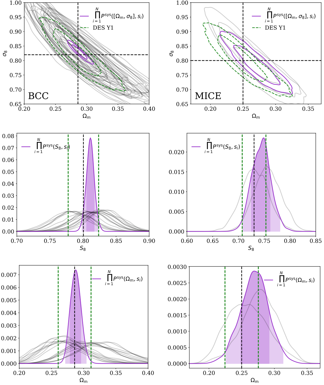
Figure 2. Cosmological constraints from all three two-point functions for the BCC (left panels, 18 realizations) and MICE (right panels, 2 realizations) simulation suites. The top panels show constraints on the present day matter density, \Omega_m and the clustering amplitude, \sigma_8 . Contours contain 68% and 95% of the posterior probability. Grey contours show constraints from individual simulation realizations, while purple contours show the combination of these posteriors (see equation 20). The middle and bottom panels show the marginalized constraints on S_8 = \sigma_8 \times (\Omega_m/0.3)^{0.5} , and \Omega_m respectively. In all panels, the true parameter values (i.e. those input to the simulations) are indicated by the black dashed lines. In the top panels, the green dashed lines indicate the 68% and 95% confidence regions recovered from the real DES Y1 data in DES Collaboration et al. (2017), shifted to be centered on the input cosmology to the simulations. In the middle and lower-panels, the green dashed lines indicate the size of the 1-\sigma uncertainty from DES Collaboration et al. (2017).
