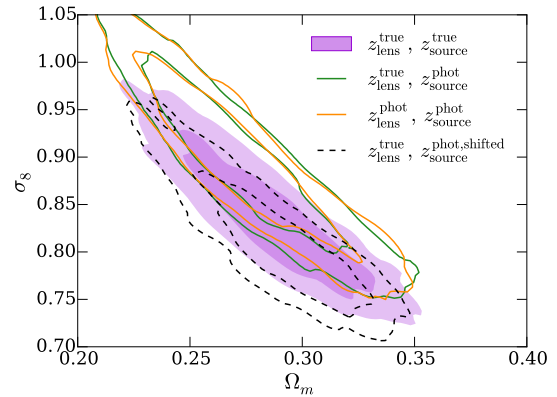
Figure 4. The impact of using photometric redshift estimates. For all contours, the datavector is the mean of all BCC realisations. Purple filled contours use the true redshift distributions for both lens and source galaxies. Note in this case galaxies are binned according to their photo- z , but the n(z) for each redshift bin is estimated using true redshifts. The green unfilled contours use source redshift distributions estimated using BPZ photo- z s, while the orange unfilled contours additionally use the photometric redshift estimates from the REDMAGIC algorithm, z_{RM} for the lenses. The black dashed contours use BPZ to estimate the source n(z) s, shifted in redshift to have the correct mean (see Section 5.4 for details).
