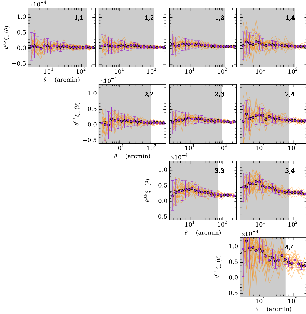
Figure A2. Measurement of \xi_-(\theta) in the BCC simulations. Dark orchid data points are the mean across all 18 simulations, while orange lines indicate measurements from individual realizations. Errorbars indicate the expected uncertainty from a single DES Y1 realization. The line is the theoretical prediction assuming the true cosmology. Grey shaded regions are excluded from the fiducial analysis.
