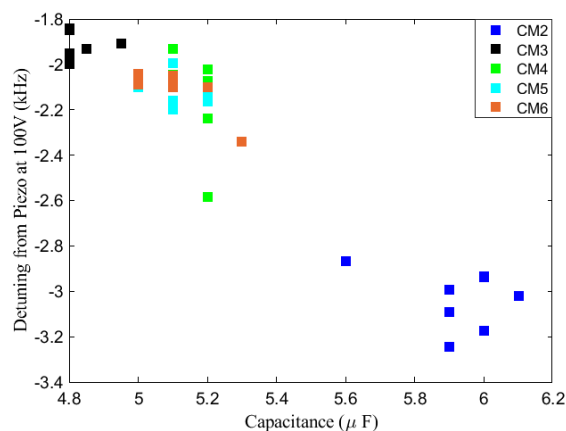
Figure 6: Piezo tuner sensitivity vs. capacitance of the piezo-actuators.
