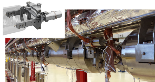
Figure 1: LCLS II cold-mass with tuners installed.
