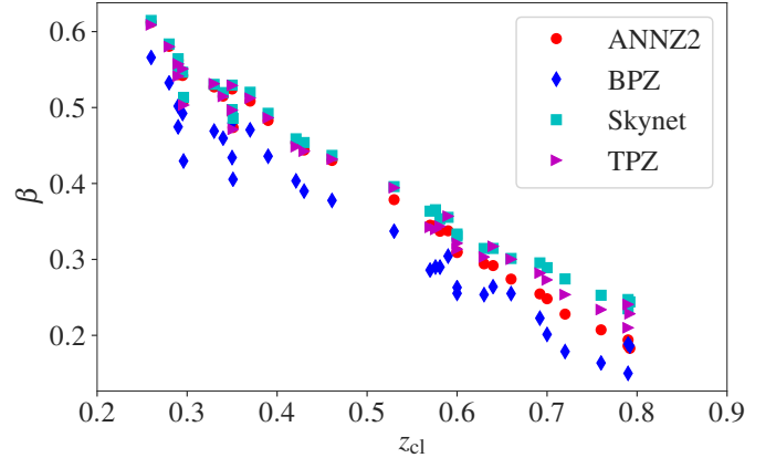
Figure A4. Estimated lensing efficiency \beta for our background source population for each cluster when employing different redshift codes. The different values are plotted against the cluster redshift z_{cl} . The three training-set based methods (ANNZ2, TPZ, and SKYNET) show the best agreement while the template based BPZ code disagrees most strongly with the fiducial SKYNET algorithm.
