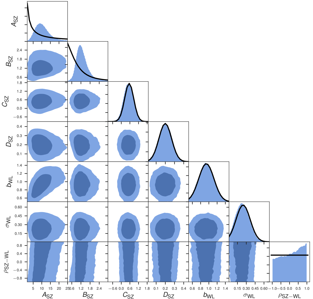
Figure 5. Scaling relation parameter constraints derived from our DES-SV WL analysis. Priors (see Section 4.2) are shown with black lines, where priors for C_{\text{SZ}} and D_{\text{SZ}} come from de Haan et al. (2016), and b_{\text{WL}} and \sigma_{\text{WL}} arise from our analysis of simulations. Parameters A_{\text{SZ}} , B_{\text{SZ}} and \rho_{\text{SZ-WL}} are given broad, uninformative priors and are thus constrained only by WL data. For A_{\text{SZ}} we find higher values than expected, though still consistent with most previous analyses. Our data prefer an approximately self-similar value for B_{\text{SZ}} , although the uncertainties are large. The data provide no evidence for a correlation between the intrinsic scatter in the SZE-mass and WL-mass scaling relations.
