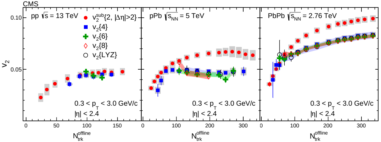
Figure 10: Left: The v_2^{\text{sub}} , v_2\{4\} and v_2\{6\} values as a function of N_{\text{trk}}^{\text{offline}} for charged particles, averaged over 0.3 < p_T < 3.0 GeV/c and |\eta| < 2.4 , in pp collisions at \sqrt{s} = 13 TeV. Middle: The v_2^{\text{sub}} , v_2\{4\} , v_2\{6\} , v_2\{8\} , and v_2\{\text{LYZ}\} values in pPb collisions at \sqrt{s_{\text{NN}}} = 5 TeV [40]. Right: The v_2^{\text{sub}} , v_2\{4\} , v_2\{6\} , v_2\{8\} , and v_2\{\text{LYZ}\} values in PbPb collisions at \sqrt{s_{\text{NN}}} = 2.76 TeV [40]. The error bars correspond to the statistical uncertainties, while the shaded areas denote the systematic uncertainties.
