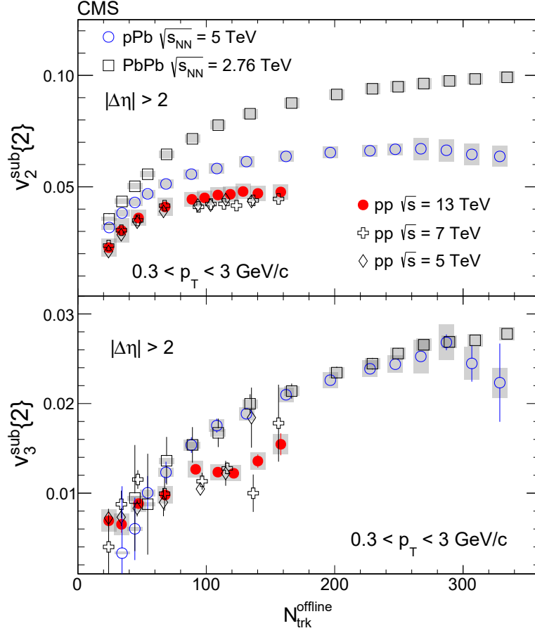
Figure 5: The v_2^{\text{sub}} (top) and v_3^{\text{sub}} (bottom) results of charged particles as a function of N_{\text{trk}}^{\text{offline}} , averaged over 0.3 < p_T < 3.0 \text{ GeV/c} , in pp collisions at \sqrt{s} = 5, 7 , and 13 \text{ TeV} , pPb collisions at \sqrt{s_{\text{NN}}} = 5 \text{ TeV} , and PbPb collisions \sqrt{s_{\text{NN}}} = 2.76 \text{ TeV} , after correcting for back-to-back jet correlations estimated from low-multiplicity data. The error bars correspond to the statistical uncertainties, while the shaded areas denote the systematic uncertainties. Systematic uncertainties are found to have no dependence on \sqrt{s} for pp results and therefore are only shown for 13 \text{ TeV} .
