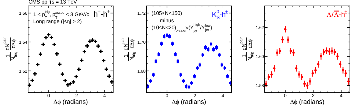
Figure 3: The 1D \Delta\phi correlation functions for the long-range regions in the multiplicity range 105 \leq N_{\text{trk}}^{\text{offline}} < 150 of pp collisions at \sqrt{s} = 13 TeV, after subtracting scaled results from 10 \leq N_{\text{trk}}^{\text{offline}} < 20 with the ZYAM procedure applied. A selection of 1–3 GeV/c for both p_T^{\text{trig}} and p_T^{\text{assoc}} is used in all cases.
