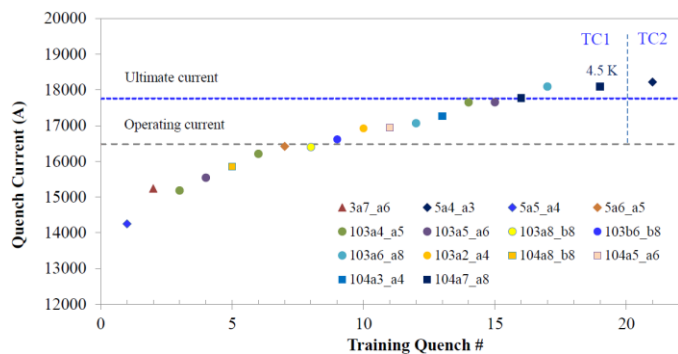
Fig. 3. MQXFS1 quench training history
