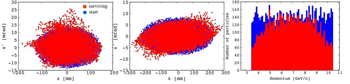
FIG. 8: Start (in blue) and surviving (red) pions \pi^+ after the FFAG double achromat bend in the bending phase space plane (left), in the non-bending phase space plane (center), and the momentum distribution (right).
