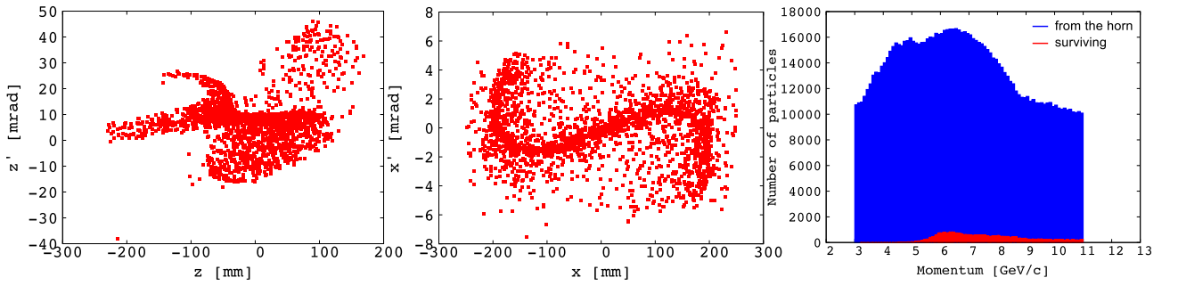
FIG. 9: Start (in blue) and surviving (red) pions \pi^- after the FFAG double achromat bend in the bending phase space plane (left), in the non-bending phase space plane (center), and the momentum distribution (right).
