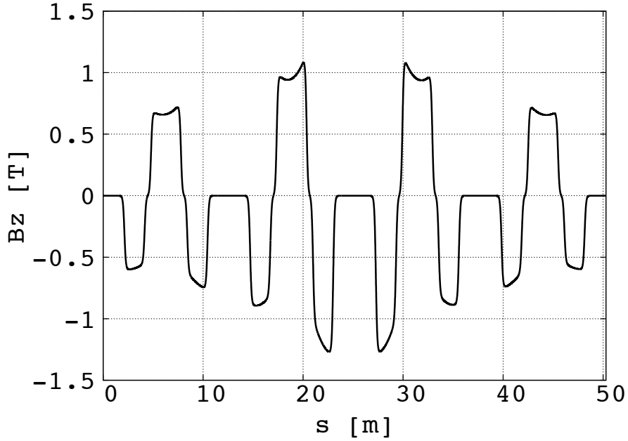
FIG. 7: Magnetic field for 10.5 GeV/c in the FFAG double achromat bend.
