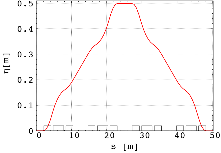
FIG. 6: dispersion function in the FFAG double achromat bend at 7 GeV/c.
