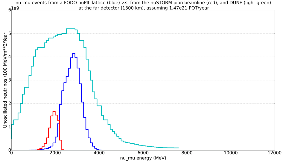
FIG. 4: Neutrino flux in the FODO solution.
