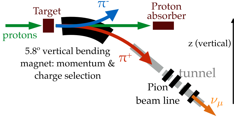
FIG. 1: Scheme of the nuPIL concept.
