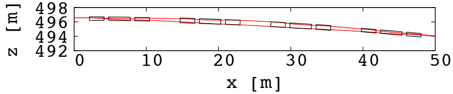
FIG. 5: FFAG double achromat bending beam line with trajectories of 3.5 GeV/c and 10.5 GeV/c in red.
