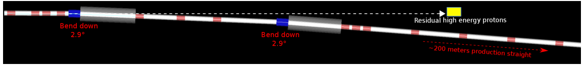
FIG. 3: FODO solution tracked in G4BL.
