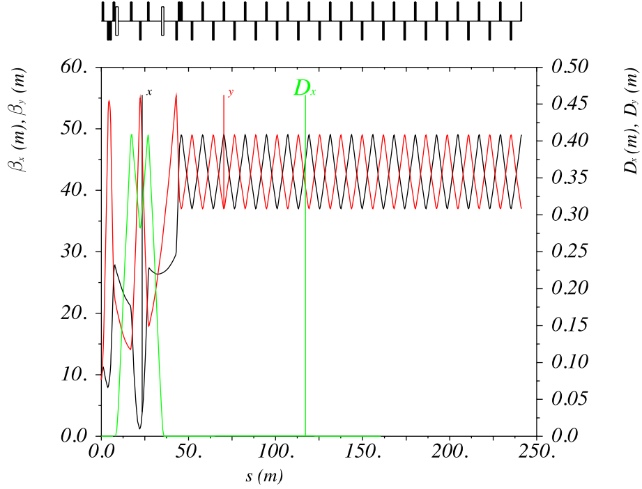
FIG. 2: linear parameters of the FoDo solution.
