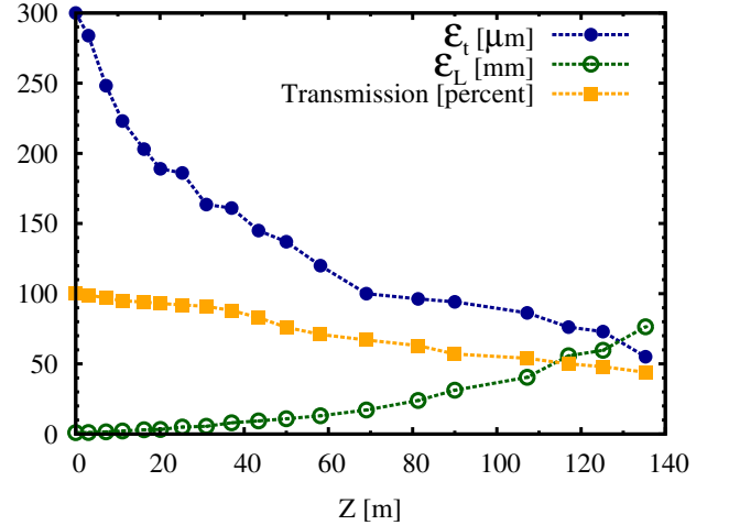
FIG. 8. Transverse and longitudinal emittance in the channel, along with the transmission which includes muon decay.
