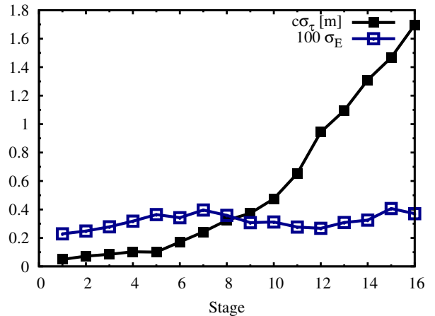
FIG. 7. Bunch length and energy spread across the channel.
