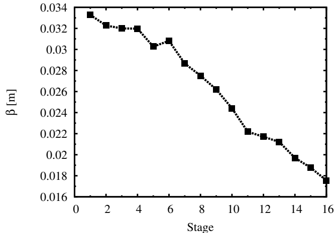
FIG. 6. Transverse Twiss \beta -function at the center of strong focusing solenoid in each stage of the 16 stages.
