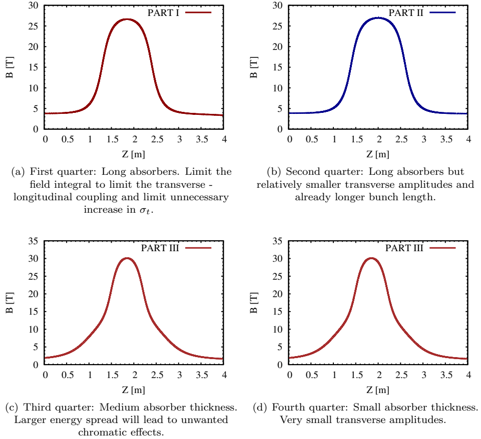
FIG. 5. On-axis field of four of the focusing solenoids used in the ionization cooling channel.
