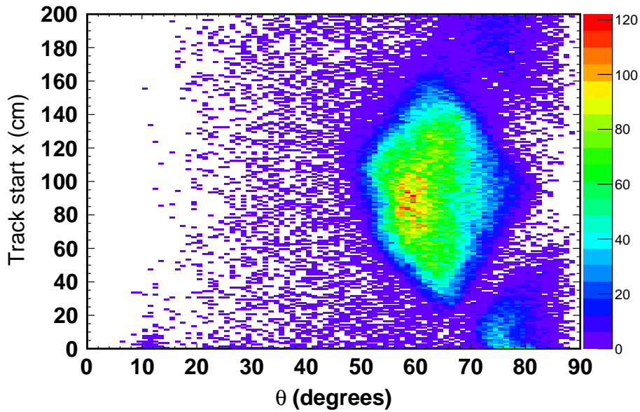
Figure 12: Reconstructed track start point in the drift direction ( x ) versus track angle ( \theta ). The muons normally enter the TPC in the middle, but they can be close to the wire planes and cathode.
