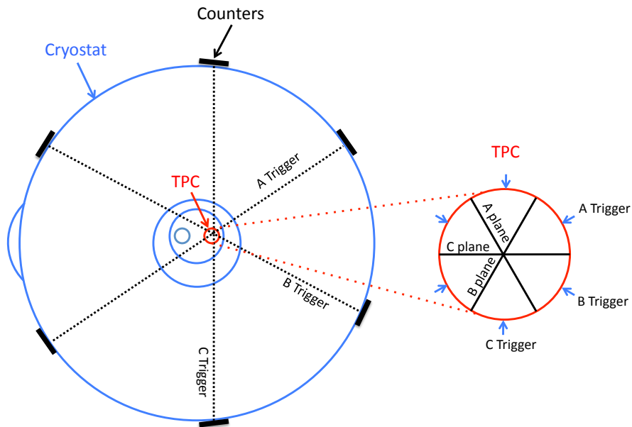
Figure 5: Location of the scintillation counters (left) and TPC wire orientations (right).
