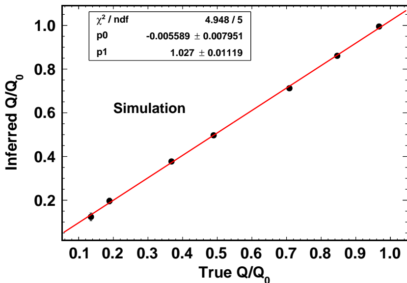
Figure 16: Q/Q_0 determined using Monte Carlo simulated events and the method described in the text compared to the value of Q/Q_0 used in the simulation.
