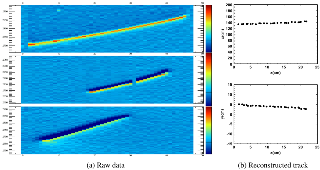
Figure 10: Run 293 Event 2225. (a) Drift time versus wire ID for raw wire signal from 3 wire planes. Red indicates positive signals and blue indicates negative signals. (b) Reconstructed track points in the x-z and y-z projections.
