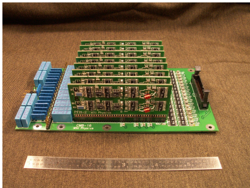
(a) Cold motherboard.
