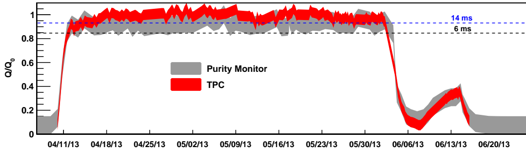
Figure 15: Comparison between Q/Q_0 measured by the TPC and the converted Q/Q_0 using the purity monitor data. Q/Q_0 is a measure of the electron lifetime, and the values \tau = 6 ms and \tau = 14 ms that correspond to Q/Q_0 = 0.85 and Q/Q_0 = 0.93 , respectively, are indicated with dashed lines.
