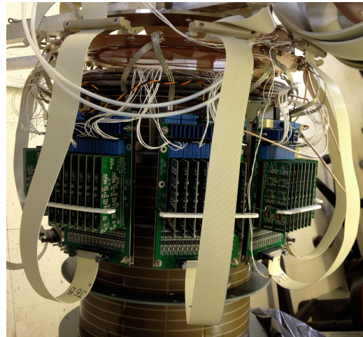
(b) TPC with preamp-filters mounted.
