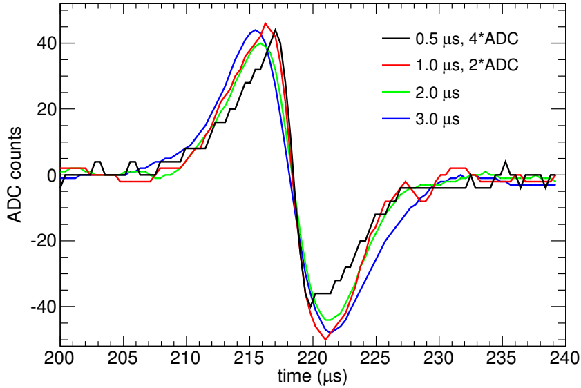
Figure 8: Raw signal shapes for induction plane signals with different settings of the ASIC shaping time constant are shown. The horizontal axis has an arbitrary zero so that the pulses are shown with the zero crossing point artificially aligned. The tracks from which these signals are taken form an angle of roughly 20 degrees with the plane of the wires, or \theta \sim 70 . The angle between the projection of the track onto the wire plane and the wires themselves is \sim 80 degrees.
