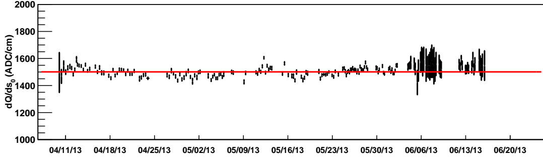
Figure 14: dQ/ds_0 as a function of time.
