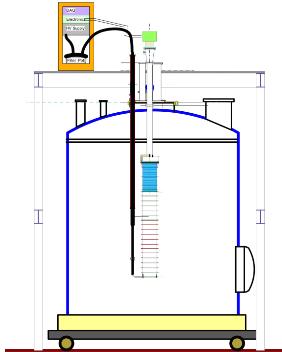
Figure 9: The TPC and high voltage feed through inside the LAPD cryostat.
