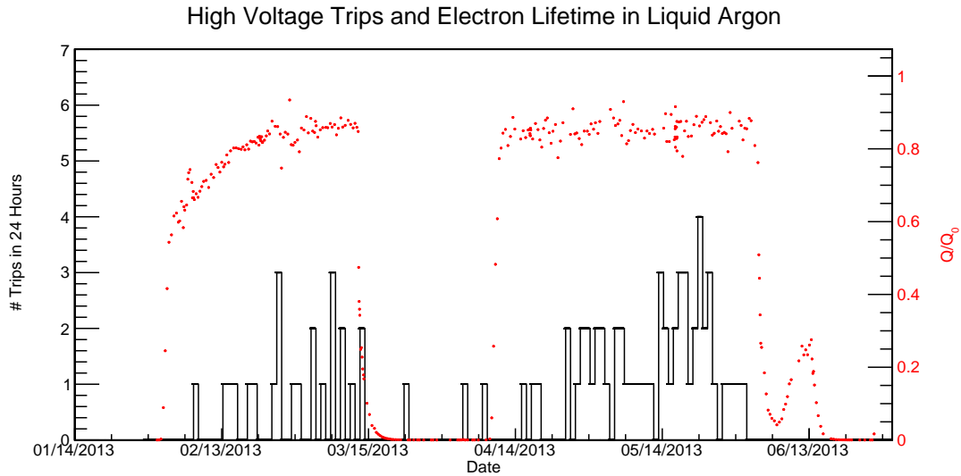
Figure 17: The number of cathode high voltage trips in a 24 hour period and purity monitor values during data taking. The trip counts are given by the black solid line and scale on the left. Trips related to testing the high voltage system were not included in the trip count. A quantification of the argon purity is given by the red dots and the scale on the right, which is the converted Q/Q_0 using purity monitor data.
