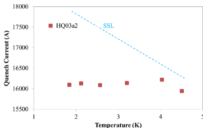
Fig. 3: Dependence of the quench current on temperature.
