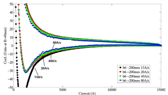
Fig. 11: Normal dodecapole as a function of the magnet current at different ramp rates.
