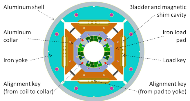
Fig. 1. LARP High Field Quadrupole (HQ) magnet cross-section.
