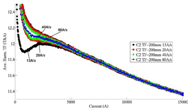
Fig. 10: Transfer function as a function of the magnet current at different ramp rates.
