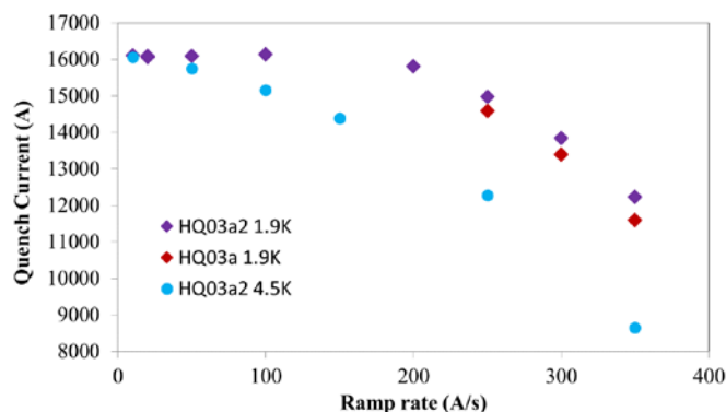
Fig. 4: Dependence of the quench current on ramp rate.
