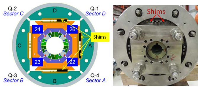
Fig. 8: Magnetic shim configuration in HQ03a.
