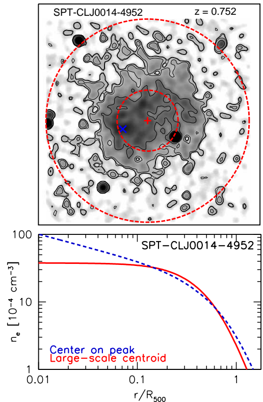
FIG. 6.— Top: Smoothed X-ray image of SPT-CLJ0014-4952. The X-ray peak and large-annulus centroid are depicted with blue and red crosses, respectively. The two red dashed circles correspond to radii of 0.3R_{500} and R_{500} . Bottom: Electron density profile, derived using the two different centers. For “disturbed” clusters the X-ray peak can be significantly offset from the large-scale centroid, leading to a deficit of core pressure ( \sim 50\% ) and slight excess pressure at large radii ( \sim 15\% ) if the latter is chosen as the cluster center.
