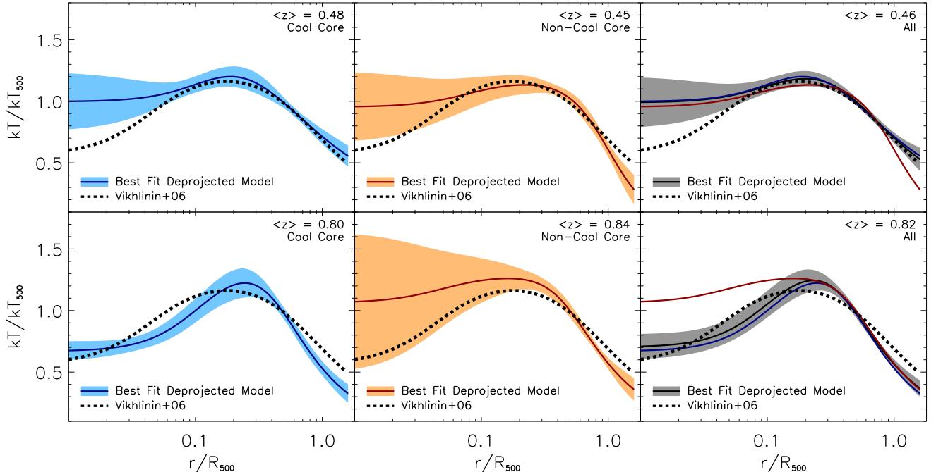
FIG. 4.— Deprojected temperature profiles for each of the six subsamples. Colored curves correspond to the best-fit deprojected model and the 1\sigma uncertainty in this model. In the right-most panels, we overplot the cool core and non-cool core profiles for comparison. In all panels we show the average deprojected temperature profile from Vikhlinin et al. (2006) for comparison. This figure highlights the lower-temperature cores and outskirts in high- z clusters, relative to their low- z counterparts. The best-fit parameters which describe these curves are provided in Table 4.
