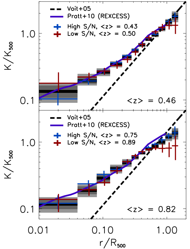
FIG. 11.— Joint-fit entropy profile for both the low- and high- z subsamples (see also Figure 7). The red and blue points correspond to the joint-fit profiles for low- and high-S/N subsamples, respectively, as described in §4.4.1. We find that, at large radii, the flattening of the entropy profile correlates with both increasing redshift and decreasing S/N. The most significant flattening is present in the high- z , low-S/N subsample, which contains 7 of the 8 clusters at z > 1 and all four z > 1.1 clusters. Given that the low- z and high- z low-S/N subsamples have similar S/N but different degrees of flattening, we propose that the observed flattening is driven primarily by increasing redshift.
