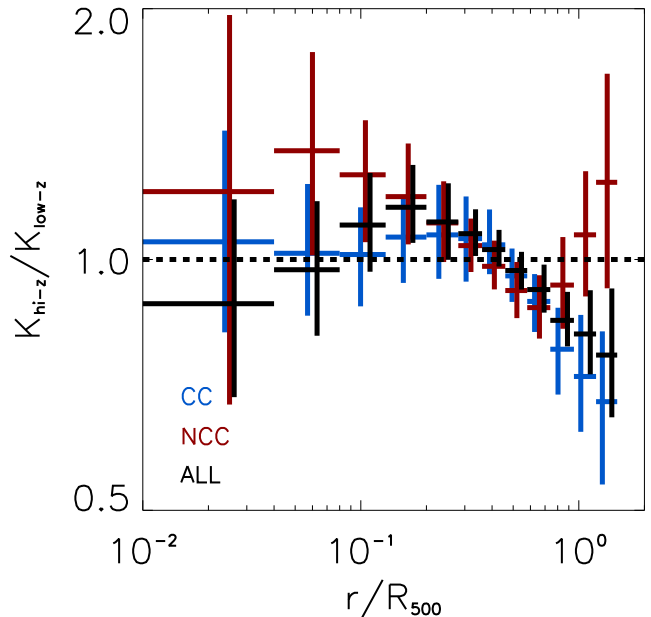
FIG. 8.— This plot compares the low- and high- z entropy profiles for three different subsamples. Here, the y-axis is the ratio of the measured entropy for the high- z subsample to the low- z subsample at a given radius. Error bars represent 1\sigma uncertainty. All three profiles are consistent with negligible evolution at r < 0.7R_{500} and significant evolution at r > 0.7R_{500} .
