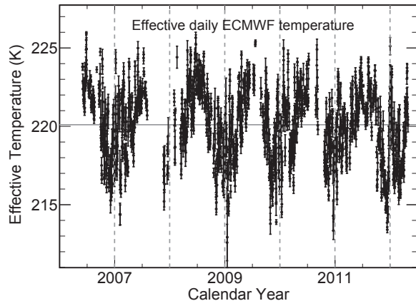
FIG. 3: Effective temperature as a function of time for the atmosphere directly above the MINOS ND. Each data point corresponds to one day of ECMWF data. The mean value is the average of the four ECMWF data points for that day. The y -axis errors are the standard deviation of those points. The solid horizontal line is the mean effective temperature \langle T_{eff} \rangle = 220.1 K. The dashed vertical lines denote the start of new calendar years.
