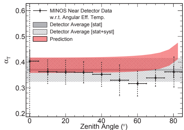
FIG. 8: The \alpha_T parameter as a function of zenith angle when T_{eff}(\theta) is calculated using Eq. (11). The inner error bars on the data points are statistical, the outer error bars include both statistical and systematic uncertainties. The gray band is the detector average calculated using T_{eff}^{weight} as defined in Eq. (12). The red band is the theoretical prediction and is the same as in Fig. 7.
