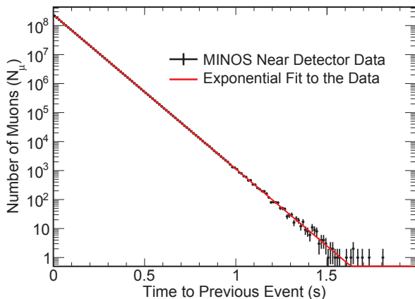
FIG. 1: Time between neighboring single atmospheric muon events in the MINOS ND. The data is well fitted to an exponential distribution with a mean rate of 12.2374 \pm 0.0003 Hz.
