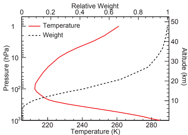
FIG. 2: The average temperature (solid red line) [14] and normalized weights W(X) (black dashed line) as a function of pressure level at the MINOS ND site. The right vertical axis shows the altitude corresponding to a particular pressure.
