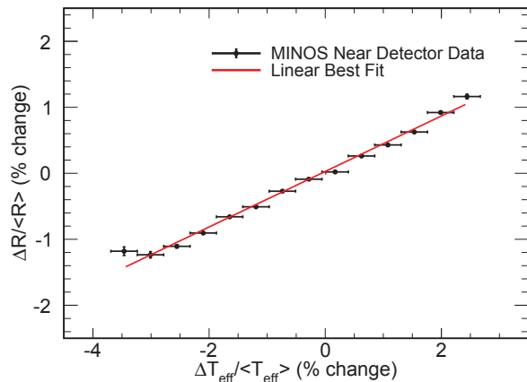
FIG. 6: The change in the observed muon rate versus the change in the effective temperature. In this Figure the muon rate has been calculated as a function of effective temperature rather than on a point-to-point basis as in Fig. 5.
