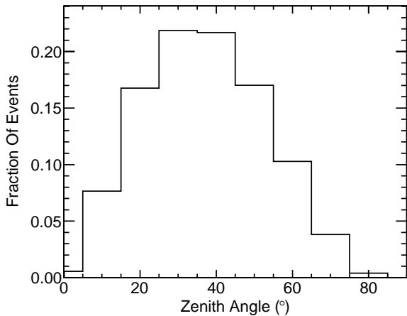
FIG. 9: Reconstructed zenith angle distribution for single muon events observed in the MINOS ND.
