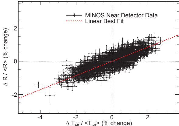
FIG. 5: Distribution of \Delta R / \langle R \rangle versus \Delta T_{eff} / \langle T_{eff} \rangle . Each data point corresponds to approximately 6 hours of MINOS ND data. The y -axis uncertainty is purely statistical. The x -axis uncertainty is 0.2% and is the point-to-point variation in the ECMWF data. The best fit slope, equivalent to \alpha_T , is 0.465 \pm 0.003(\text{stat.}) . To reduce clutter, only every fifth data point is shown.
