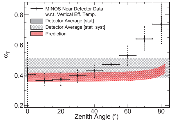
FIG. 7: The parameter \alpha_T as a function of zenith angle when T_{eff} is calculated using Eq. (2). The inner error bars on the data points are statistical, the outer error bars include both statistical and systematic uncertainties. The gray band is the detector average, and the red-band is the theoretical prediction. The systematic difference of the data from the average suggests that the vertical effective temperature is inadequate for data over a range of zenith angles.
