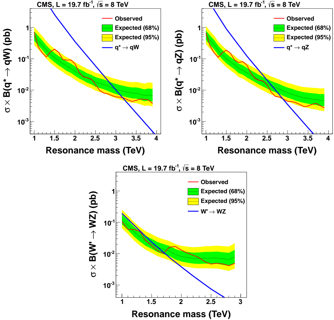
Figure 7: Expected and observed limits on the production cross section as a function of the resonance mass for (upper left) qW resonances, (upper right) qZ resonances, and (bottom) WZ resonances, compared to their predicted cross sections for the corresponding benchmark models.
