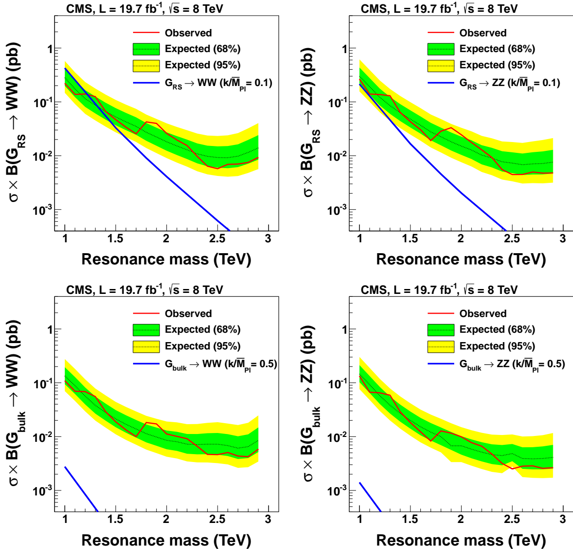
Figure 8: Expected and observed limits on the production cross section as a function of the resonance mass for (upper left) G_{RS} \rightarrow WW resonances, (upper right) G_{RS} \rightarrow ZZ resonances, (bottom left) G_{bulk} \rightarrow WW resonances, and (bottom right) G_{bulk} \rightarrow ZZ resonances, compared to the predicted cross sections.
