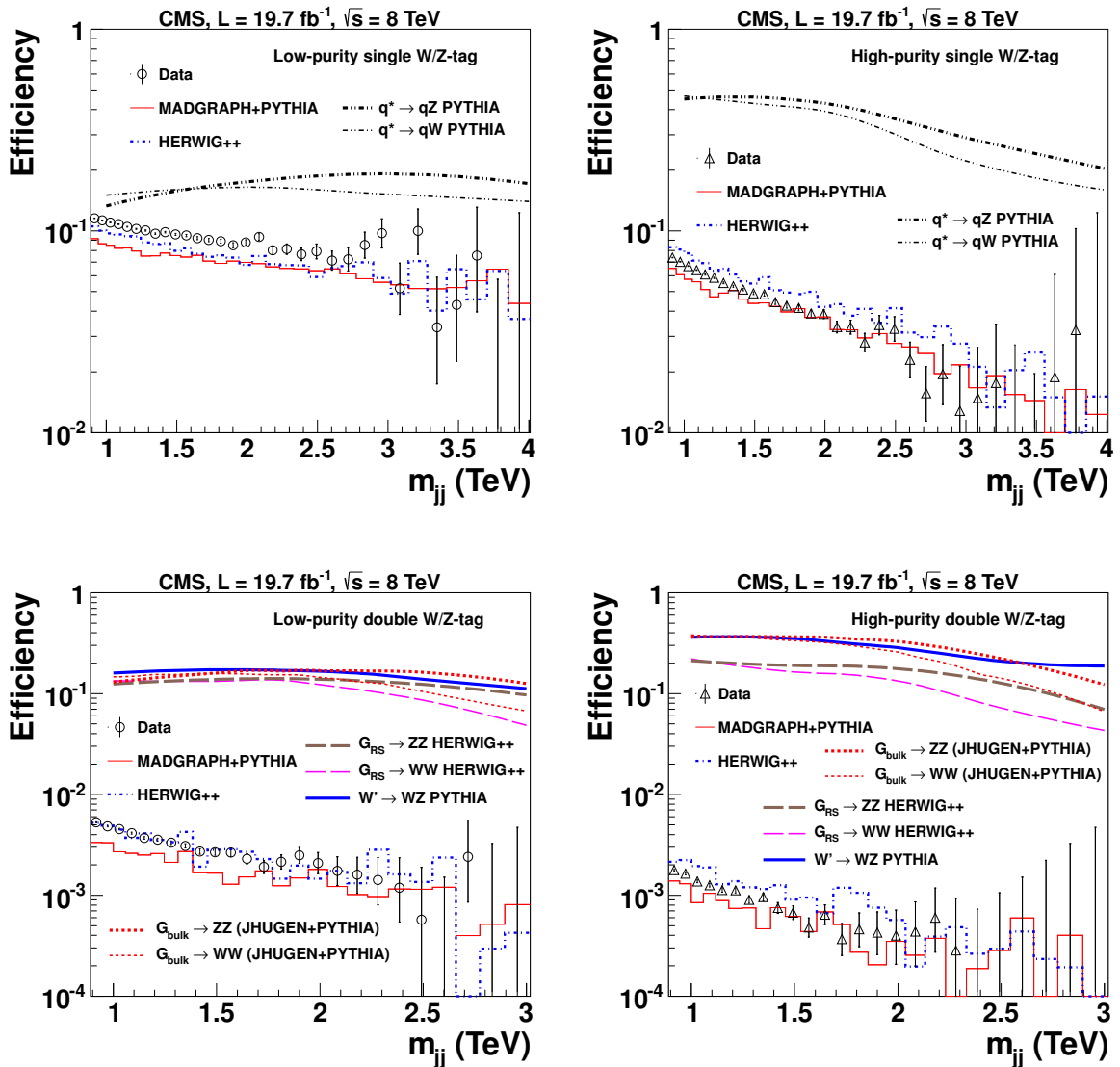
Figure 3: Efficiency of W and Z selections as a function of m_{jj} in data, and in simulations of signal and background events, with (upper left) one LP or (upper right) HP W/Z-tag, and the fraction of (lower left) doubly-tagged events in the LP and (lower right) HP category. The efficiency is computed for W/Z \rightarrow \bar{q}q' \rightarrow \text{jets} events, where the jets have |\eta| < 2.5 and |\Delta\eta| < 1.3 . MADGRAPH/PYTHIA and HERWIG++ refer to QCD multijet event simulations.
