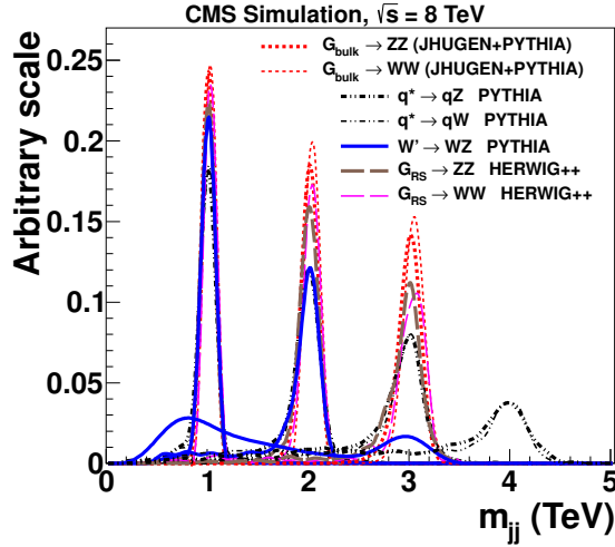
Figure 5: Distribution in m_{jj} expected in the HP categories for models corresponding to the resonance masses of 1, 2, 3, and 4 TeV. All distributions are normalized to the same area.
