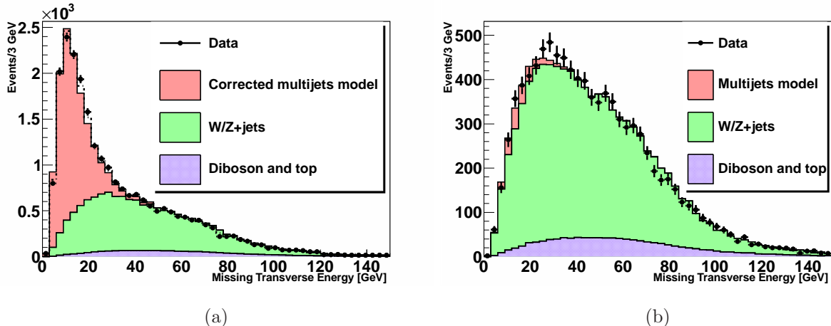
FIG. 6. Missing transverse-energy distribution for events containing electrons (a) and muons (b) from the selected sample. The distributions of observed data are shown with fit background overlaid.
