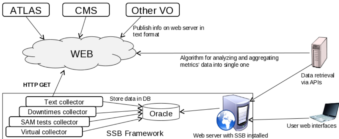
Figure 2 Data flow of SSB
