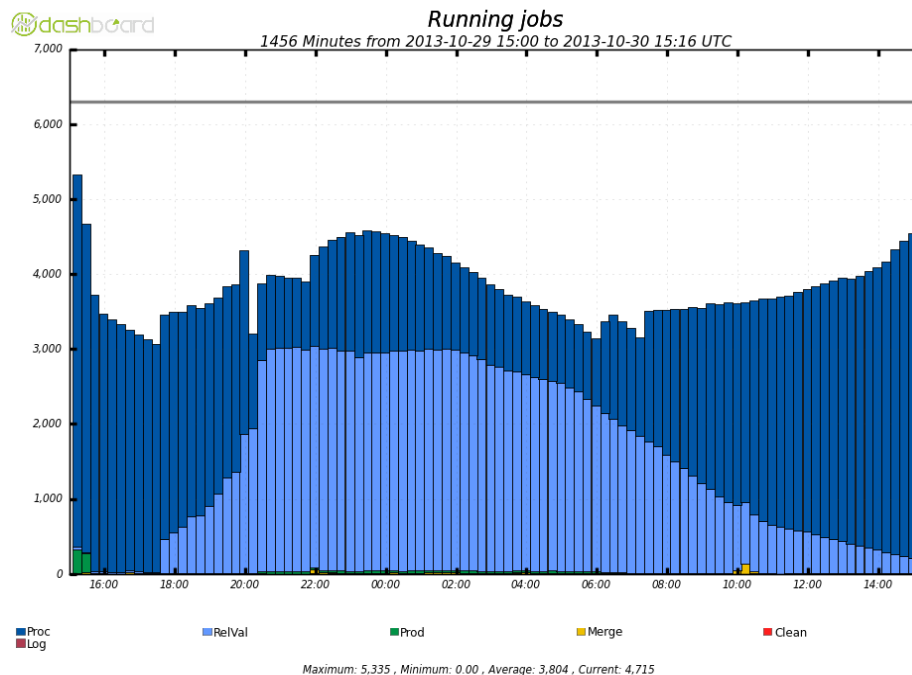
Figure 1 SSB plot showing number of production running jobs at a site including pledged slots
