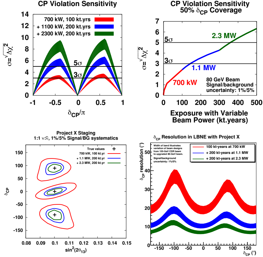
Figure 10: CP-violation sensitivity as a function of \delta_{CP} (top left) and exposure for 50% coverage of the full \delta_{CP} range (top right). Also shown are the projected precision on the measurement of \delta_{CP} for various true points in the \delta_{CP} - \sin^2 2\theta_{13} plane (bottom left) and as a function of \delta_{CP} (bottom right). All plots show the increasing precision possible in a staged long-baseline neutrino program in LBNE starting from nominal 700-kW running (red), through 1.1 MW using Project X Stage 1 (blue), to 2.3 MW with Project X Stage 2 (green). Figures from [87, 113].
