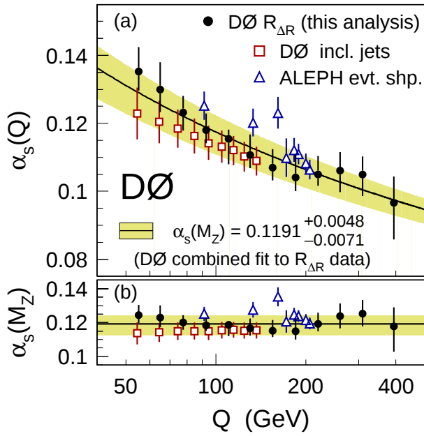
FIG. 3: (Color online.) The strong coupling \alpha_s at large momentum transfers, Q , presented as \alpha_s(Q) (a) and evolved to M_Z using the RGE (b). The uncertainty bars indicate the total uncertainty, including the experimental and theoretical contributions. The new \alpha_s results from R_{\Delta R} are compared to previous results obtained from inclusive jet cross section data [36] and from event shape data [40]. The \alpha_s(M_Z) result from the combined fit to all selected data points (b) and the corresponding RGE prediction (a) are also shown.
