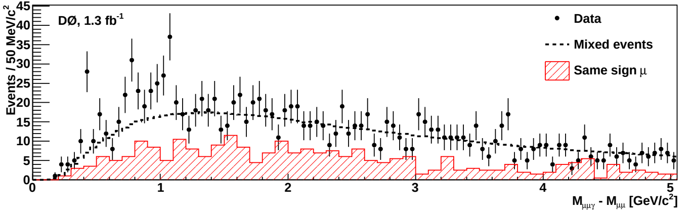
FIG. 3: Mass difference M_{\mu\mu\gamma} - M_{\mu\mu} for events passing all selection criteria. The curve shows the mass difference for the background model which combines \Upsilon(1S) and \gamma candidates from different events, normalized to the number of data events above 1.2 \text{GeV}/c^2 . The hatched area shows the distribution obtained by repeating the event selection using muons with the same charge instead of those of opposite charge.
