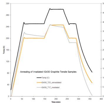
Figure 7: Annealing of irradiated IG-430 graphite
