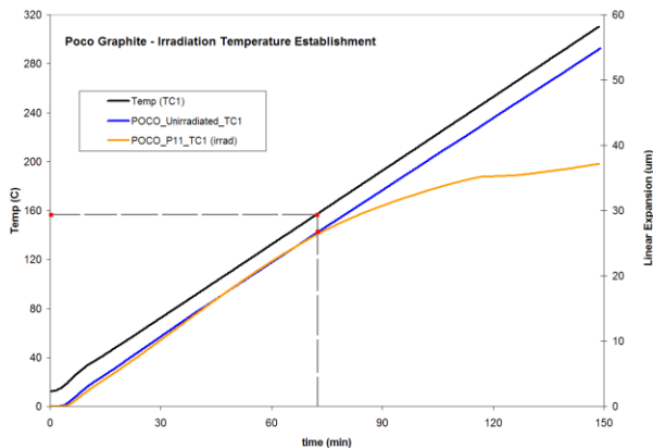
Figure 3: Post-irradiation assessment of temperature
