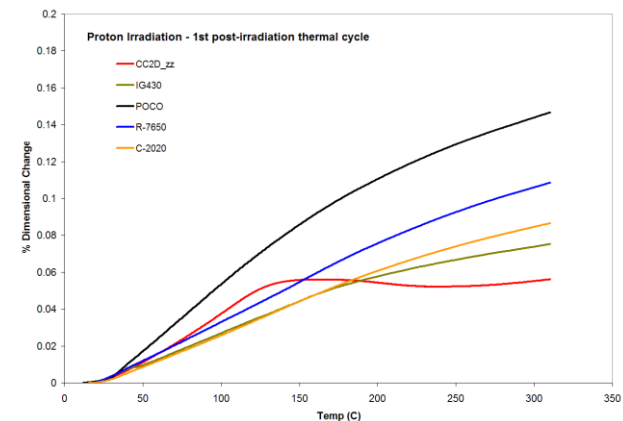
Figure 5: Dimensional change in irradiated graphites
