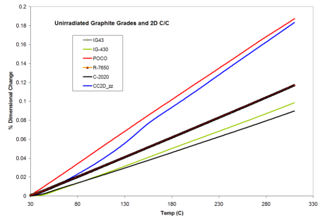
Figure 4: Unirradiated dimensional change of graphite
