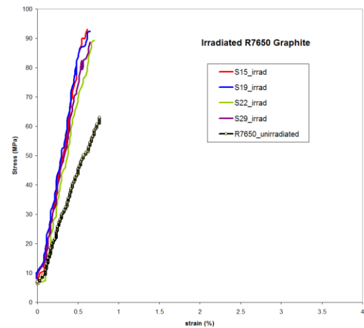
Figure 14: Stress-strain and hardening of R7650 graphite
