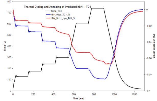
Figure 9: Irradiated h-BN annealing process
