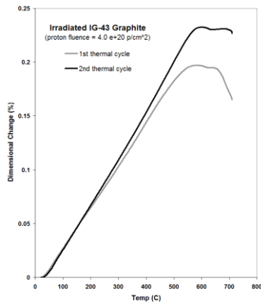
Figure 11: High temperature annealing of graphite IG-43
