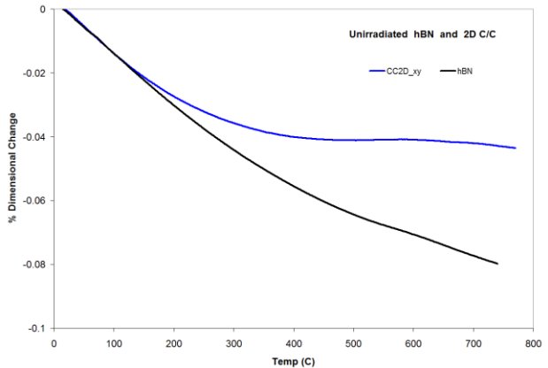
Figure 10: h-BN and fiber orientation of C/C
