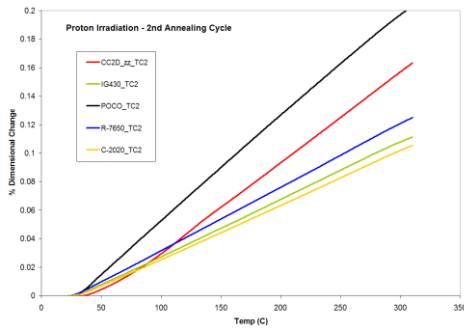
Figure 6: Achieved annealing of irradiated graphite
