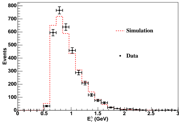
FIG. 3: (Color online) The reconstructed energy spectrum for simulation versus data in the anti-neutrino-mode \text{CC}1\pi^+ sample. Simulation is normalized to data, and only statistical errors are shown.
