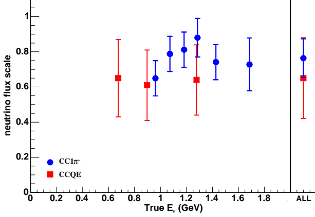
FIG. 6: (Color online) Summary of the neutrino flux constraint in the anti-neutrino-mode beam from the CC1 \pi^+ (Section IV) and CCQE (Section V) measurements.
