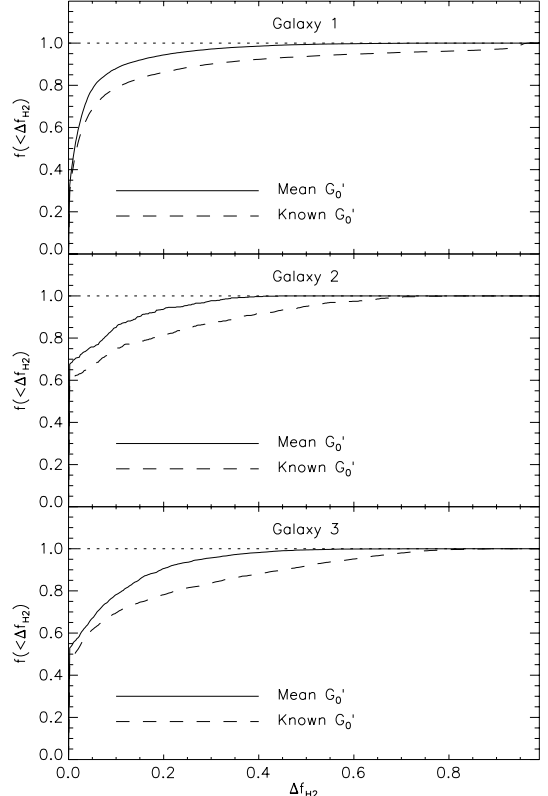
FIG. 5.— Same as Figure 1, but for the three sample galaxies with self-consistently computed radiation fields and \text{H}_2 fractions. Dashed lines show the result when we compute f_{\text{H}_2} in the KMT model using the local radiation field in each cell, while solid lines show the result when we compute f_{\text{H}_2} in the KMT model without using any information about the local radiation field, and we instead use the mean radiation field given by equation (4).
