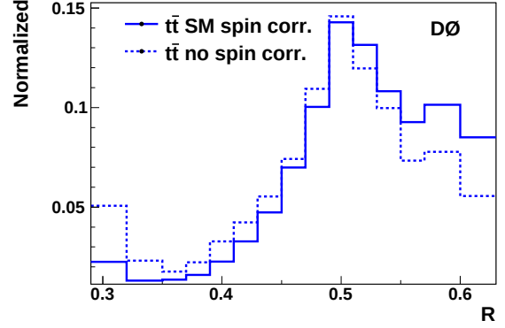
FIG. 1: Comparison of the discriminant R between SM spin correlation H = c and no spin correlation H = u at parton level. The first and last bin include also the contributions from R < 0.29 and R > 0.63 .
