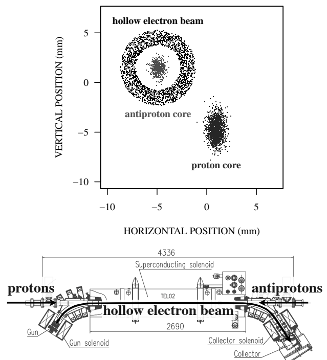
FIG. 1. Layout of the beams in the Tevatron.
