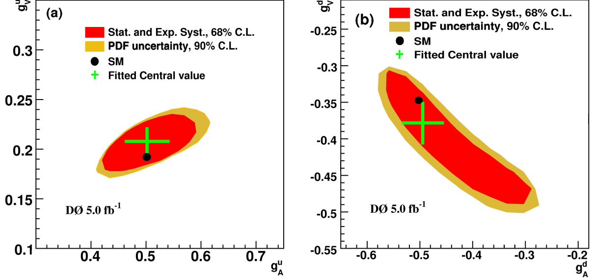
FIG. 8: (color online) The 68% C.L. contours of (a) g_V^u and g_A^u , and (b) g_V^d and g_A^d from a 2-dimensional \chi^2 fit with statistical and systematic uncertainties. The outer region is determined by the theoretical PDF uncertainty. The SM values are also shown, the crosses indicate the best fit values, and the uncertainties correspond to the 1-dimensional limits.
