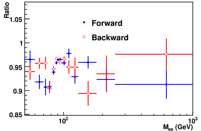
FIG. 3: The data/MC ratio of electron selection efficiencies as a function of invariant mass, for forward and backward events.
