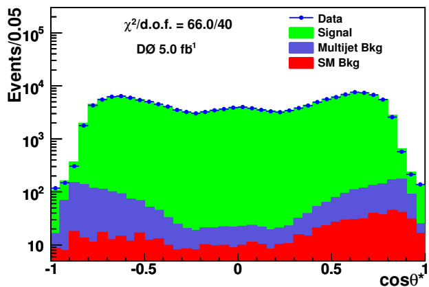
FIG. 5: Comparisons of the \cos \theta^* between data and the sum of signal and background predictions for combined CC and CE events.
