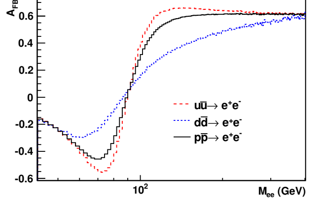
FIG. 2: The SM LO A_{FB} prediction as a function of the dielectron invariant mass for u\bar{u} \rightarrow e^+e^- , d\bar{d} \rightarrow e^+e^- , and p\bar{p} \rightarrow e^+e^- [4].
