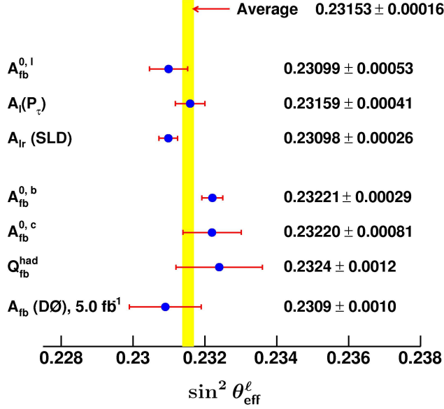
FIG. 6: Comparison of measured \sin^2 \theta_{eff}^\ell with results from other experiments. The average is a combination of A_{FB}^{0,\ell} , A_l(P_\tau) , A_{lr}(SLD) , A_{FB}^{0,b} , A_{FB}^{0,c} , and Q_{FB}^{had} measurements from the LEP and SLD Collaborations.
