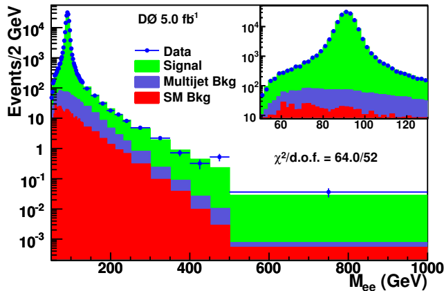
FIG. 4: Comparisons of the dielectron invariant mass between data and the sum of signal and background predictions for combined CC and CE events. The insert focuses on the Z pole region from 50 GeV to 130 GeV, where good agreement between data and the sum of signal and background predictions is essential to perform the unfolding.
