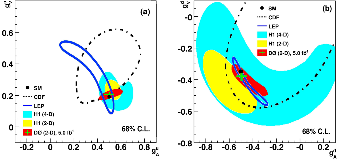
FIG. 9: (color online) The 68% C.L. contours of (a) g_V^u and g_A^u , and (b) g_V^d and g_A^d measured by DØ compared with other experiments. The LEP and CDF Collaborations performed a 4-dimensional fit ( u quark and d quark couplings simultaneous vary) to determine these couplings, while our results are 2-dimensional ( u quark ( d quark) couplings are fixed to their SM values when fitting d quark ( u quark) couplings). The H1 Collaboration performed both, a 4-dimensional and a 2-dimensional fit. The LEP results have another solution (not shown) which is excluded by the hadron collider results.
