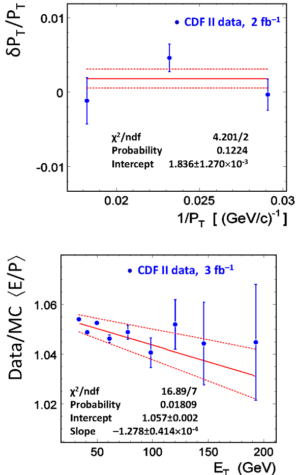
FIG. 4: Top: The constant term fit of the muon relative change of scale \delta P_T/P_T as a function of 1/P_T for Z \rightarrow \mu^+\mu^- data. Bottom: The linear fit of the data to MC ratio of the electron average E/P over each E_T bin for e + 1 jet data and MC. In each plot, the dashed lines represent \pm 1\sigma variations of the respective fit.
