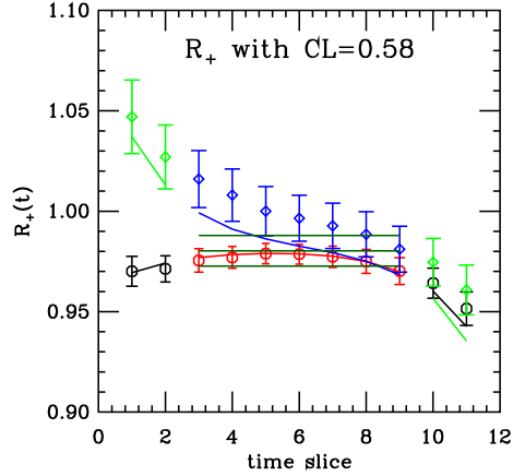
Figure 2: A sample fit to R_+(t, T; \mathbf{p}) . Example three-point correlation fit for the 0.12 fm 0.14 m_l/m_h ensemble. The circles correspond to the local source, and diamonds, the smeared source. The fit result is obtained by a simultaneous fit to both correlators using Eq. (3.3). The horizontal lines represent the central value and error of the result for R_+(\mathbf{p}) .
