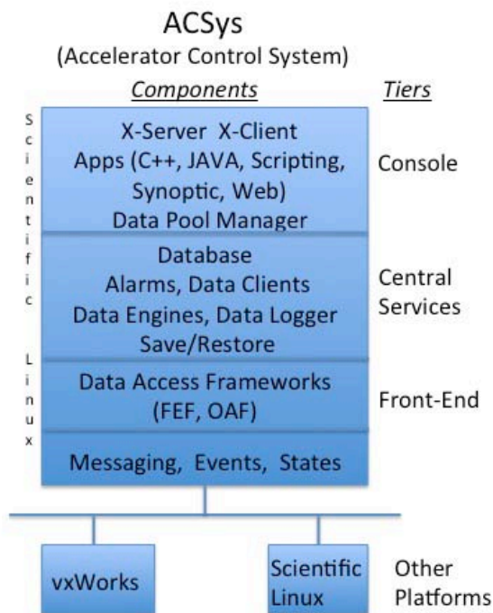
Figure 1: ACSys Configuration.
