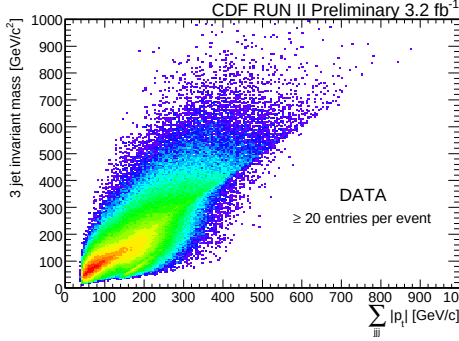
Fig. 9. – Distributions of M_{jjj} versus \Sigma_{jjj}|p_T| multiple entry( \geq 20 ).data,
