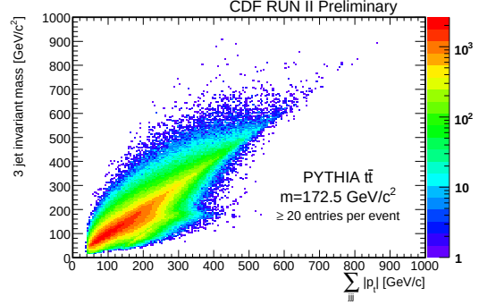
Fig. 10. – Distributions of M_{jjj} versus \Sigma_{jjj}|p_T| multiple entry( \geq 20 ).pythia t\bar{t} ( m=172.5\text{ GeV}/c^2 ),
