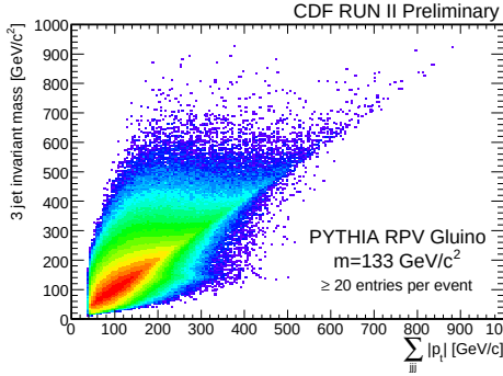
Fig. 11. – Distributions of M_{jjj} versus \Sigma_{jjj}|p_T| multiple entry( \geq 20 ).pythia RPV gluino ( m=133\text{ GeV}/c^2 ),
