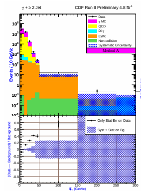
Fig. 7. – Missing Energy distribution for \gamma \pm 2 jet, CDF collaboration.
