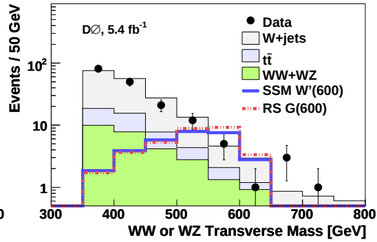
Fig. 5. – Reconstructed WZ or WW transverse mass in the \nu\bar{\nu}jj channel, D0 collaboration.
