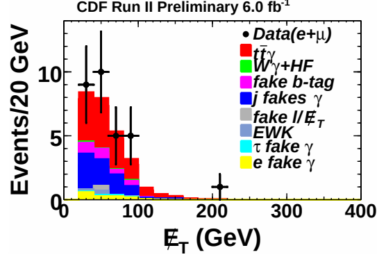
Fig. 8. – Missing Energy distribution in 1\gamma MET b events, CDF collaboration.
