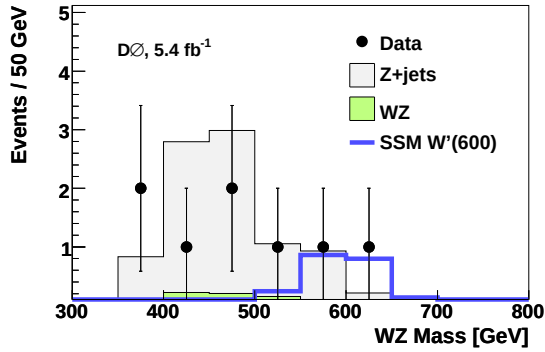
Fig. 4. – Reconstructed WZ mass in the \nu\text{jj} , \text{lljj} , \text{ll}\nu channels, D0 collaboration.
