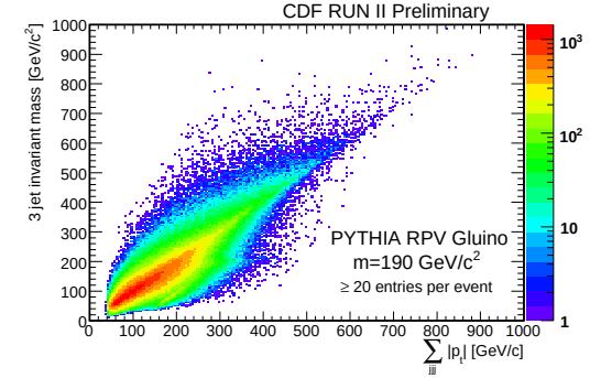
Fig. 12. – Distributions of M_{jjj} versus \Sigma_{jjj}|p_T| multiple entry( \geq 20 ).pythia RPV gluino ( m=190\text{ GeV}/c^2 )
