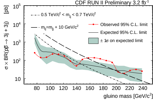
Fig. 13. – The observed and expected limit including systematic uncertainties as well as the theory cross section for \sigma(p\bar{p} \rightarrow XX) \times Br(\tilde{g}\tilde{g} \rightarrow 3jets + 3jets) where X = \tilde{g}, \tilde{q} , versus gluino invariant mass. The RPV gluino cross-section is from PYTHIA and is corrected by an NLO k-factor.
