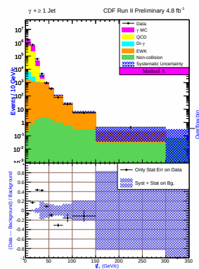
Fig. 6. – Missing Energy distribution for \gamma \pm 1 jet, CDF collaboration.
