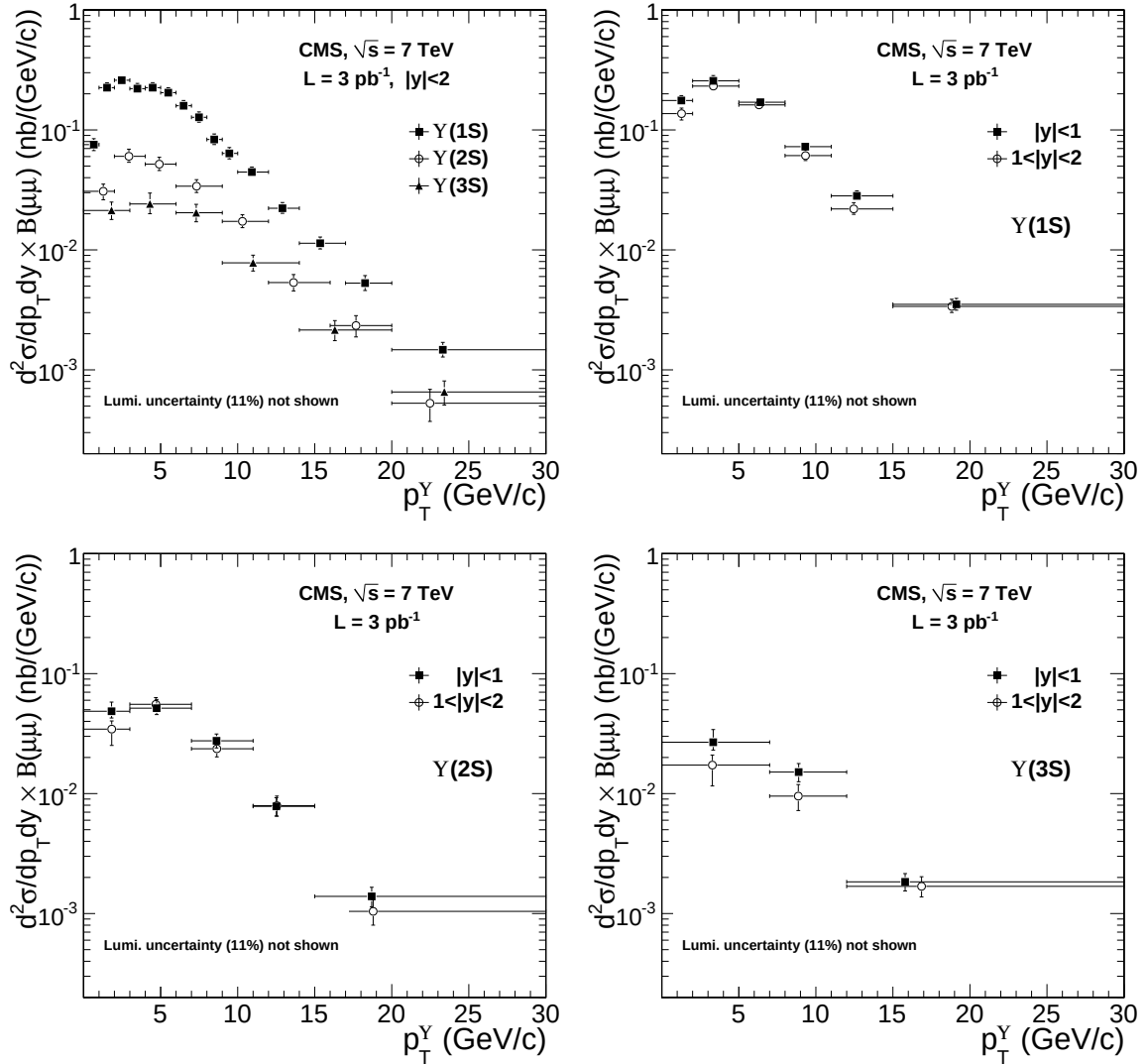
Figure 6: Y(nS) differential cross sections in the rapidity interval |y| < 2 (top left), and in the rapidity intervals |y| < 1 and 1 < |y| < 2 for the Y(1S) (top right), Y(2S) (bottom left) and Y(3S) (bottom right). The uncertainties on the points represent the sum of the statistical and systematic uncertainties added in quadrature, excluding the uncertainty on the integrated luminosity (11%).
