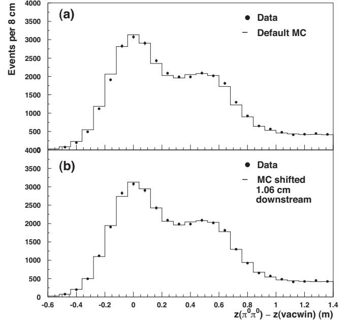
FIG. 16: z -vertex distributions of \pi^0 \pi^0 pairs produced hadronically in downstream detector elements for 1999 data and MC. (a) Data (dots) and nominal MC (histogram). (b) Data (dots) and MC that is shifted 1.06 cm downstream to match the data (histogram).
