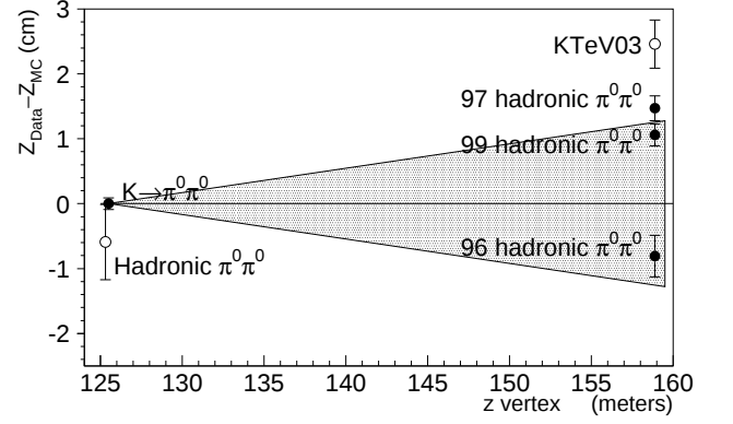
FIG. 15: Energy scale tests at the regenerator and vacuum window. The difference between the reconstructed z positions for data and MC is plotted for K \rightarrow \pi^0 \pi^0 events, and for hadronically produced \pi^0 \pi^0 pairs at the regenerator and the downstream detector elements. The solid point at the regenerator edge is the K \rightarrow \pi^0 \pi^0 sample; there is no difference between data and MC by construction. The open point at the regenerator edge is the average shift of the hadronic regenerator samples for all three datasets. The points at the vacuum window are the shifts for the downstream hadronic events for each dataset separately. The shaded region shows the range of data-MC shifts covered by the total systematic uncertainty from the energy scale. For reference, the data-MC shift at the vacuum window from KTeV03 is also plotted.
