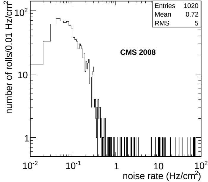
Figure 5: Example distribution of the number of rolls as a function of the average noise in the roll, for a given data taking run. Channels exceeding 100 Hz/cm 2 are masked and do not contribute to the average noise. The operating voltage is 9.2 kV.
