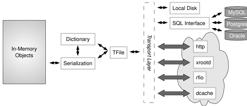
Fig. 3. Transient/persistent conversion in ROOT.
