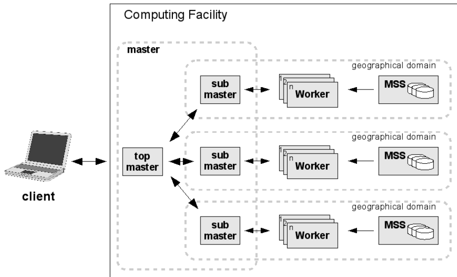
Fig. 10. PROOF multi-tier master-worker architecture.
