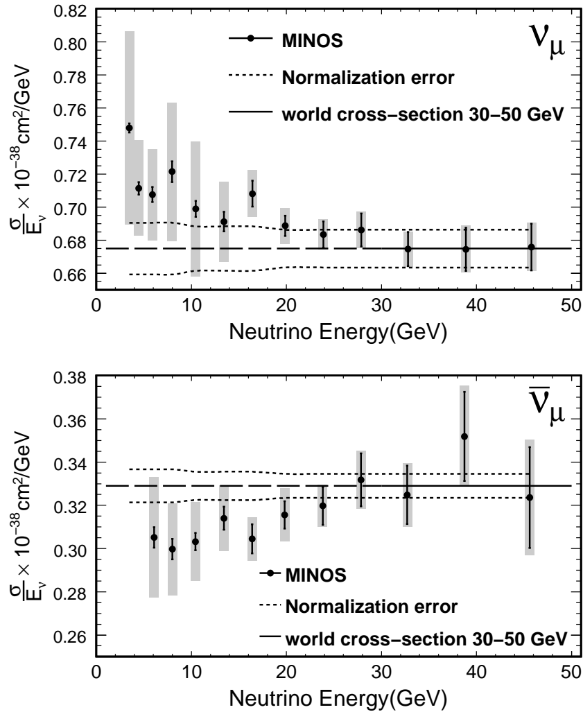
FIG. 10: Neutrino (top) and antineutrino (bottom) charged-current inclusive cross section per nucleon divided by energy for an isoscalar iron target. The black error bars show the statistical uncertainty and the shaded boxes show the statistical and systematic uncertainties added in quadrature. The dotted band shows the uncertainty on the normalization (about 1.5%). The solid black line shows the world average neutrino cross section value of 0.675 \times 10^{-38} \text{ cm}^2/\text{GeV} from 30 to 50 GeV [1–3, 11, 17] and the dashed black line shows this value extrapolated to lower energies. The neutrino cross section above 30 GeV is normalized using this world average value and the same normalization constant is then applied to the antineutrinos. The solid black line on the antineutrino cross section plot shows a world average antineutrino cross section value of 0.329 \times 10^{-38} \text{ cm}^2/\text{GeV} from 30 to 50 GeV [2, 3, 11]. This value is shown for comparison and is not used for antineutrino sample normalization.
