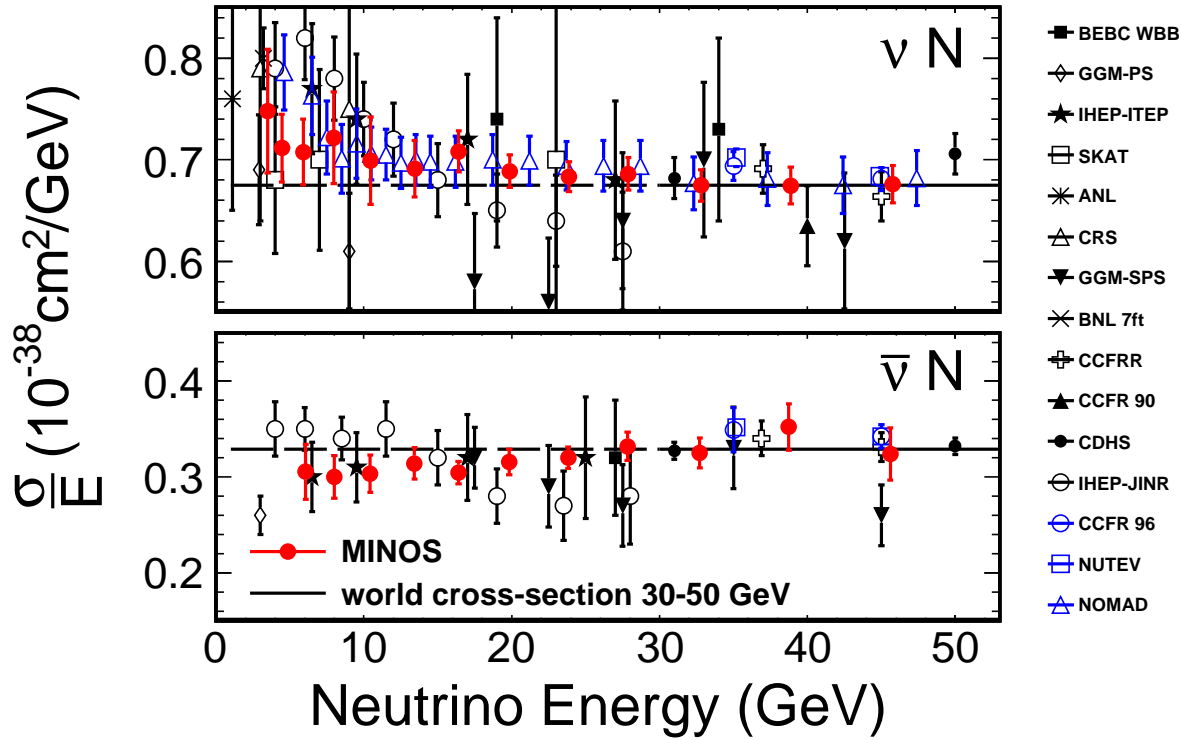
FIG. 11: MINOS neutrino and antineutrino charged-current inclusive cross section compared with other experimental results [1–3, 8–13, 15, 17–20, 45, 46]. The error bars show the statistical, systematic, and normalization uncertainties added in quadrature. The solid black line shows the average world cross section in the 30 to 50 GeV region for the neutrino ( 0.675 \times 10^{-38} \text{ cm}^2/\text{GeV} ) and the antineutrino ( 0.329 \times 10^{-38} \text{ cm}^2/\text{GeV} ). The dashed line shows these high energy values extrapolated to lower energies.
