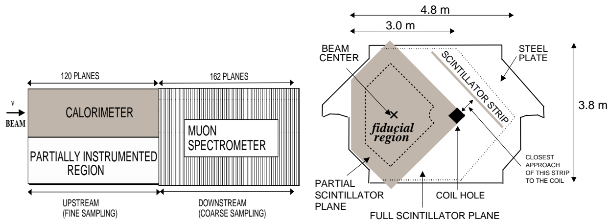
FIG. 2: Left: top view of the Near Detector, showing the calorimeter and muon spectrometer. The drawing is not to scale. Right: transverse view of a Near Detector plane. The shaded area shows a partially instrumented active scintillator plane and the dashed line within shows the boundary of the fiducial region. The dotted line shows the outline of a fully instrumented scintillator plane.
