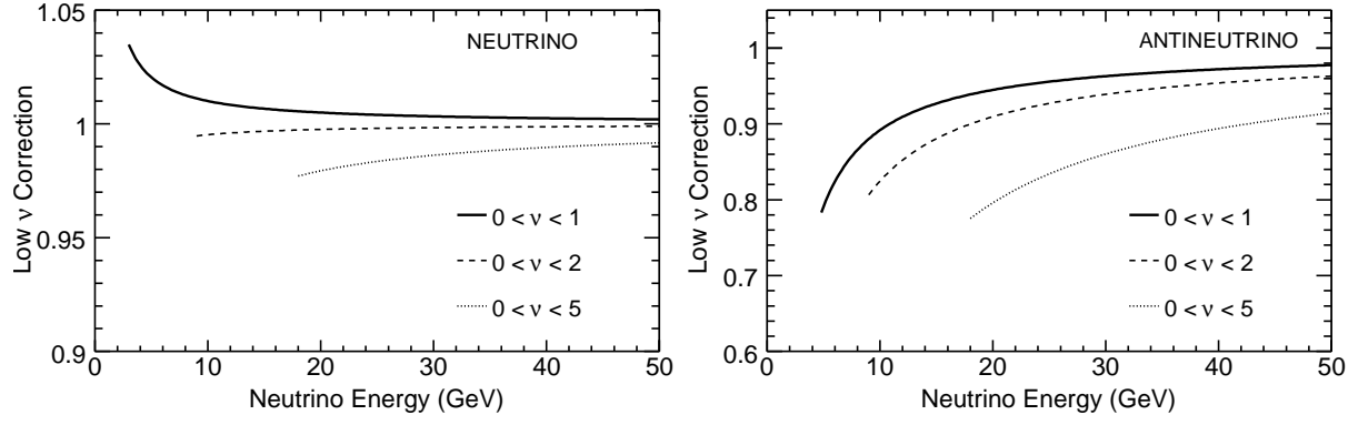
FIG. 5: The low- \nu correction, S^{\nu(\bar{\nu})}(E) , applied to the flux sample for neutrinos (left) and antineutrinos (right). The solid line shows S^{\nu(\bar{\nu})}(E) for \nu < 1 GeV applied from 3-9 GeV (5-9 GeV for \bar{\nu} ), dashed line for \nu < 2 GeV applied from 9-18 GeV, and the dotted line for \nu < 5 GeV applied above 18 GeV.
