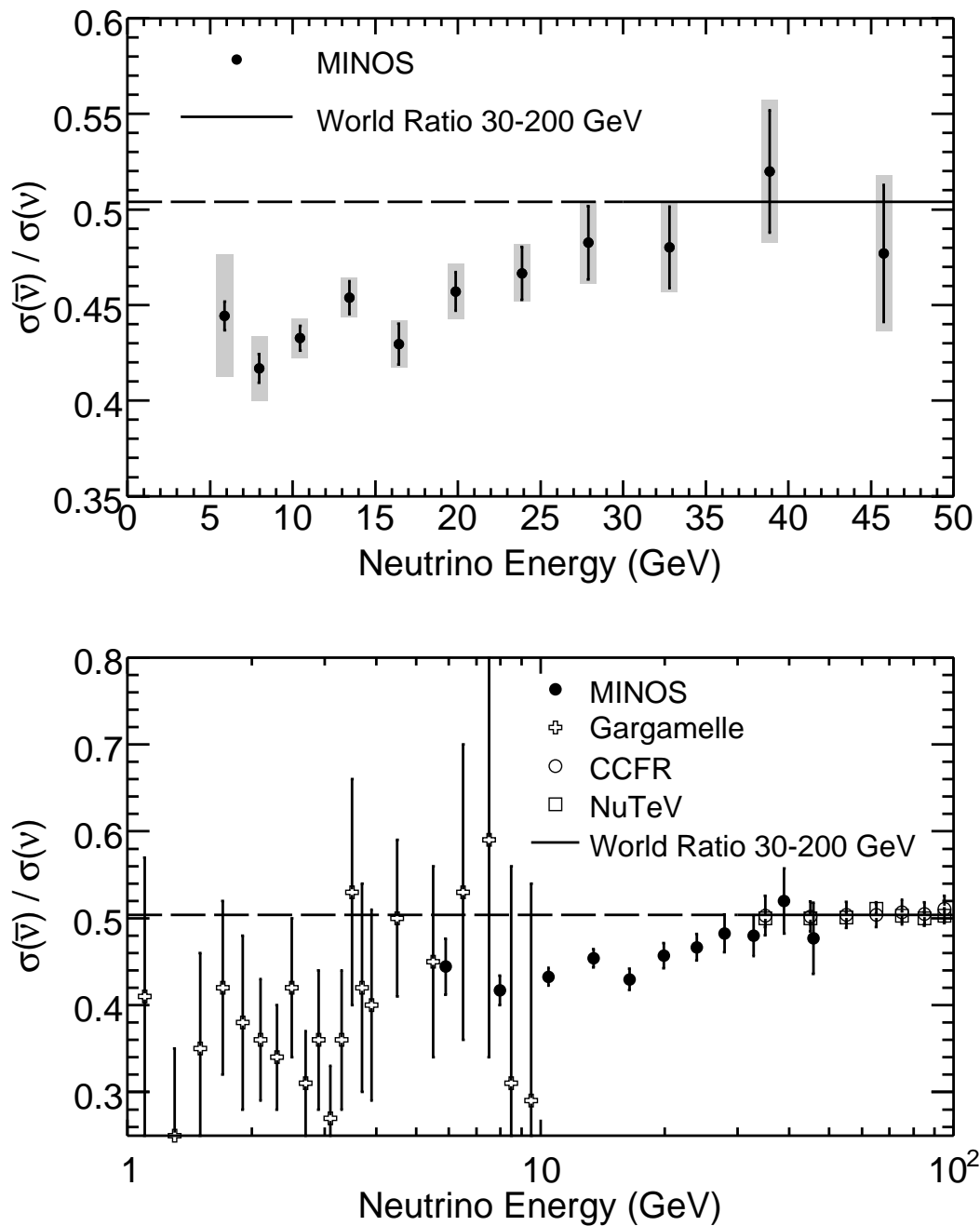
FIG. 12: (top) Ratio of antineutrino-nucleon to neutrino-nucleon cross section as a function of energy. Black error bars show the statistical uncertainty and shaded boxes show the total uncertainty with statistical and systematic uncertainties added in quadrature. The solid black line at 0.504 \pm 0.003 is drawn at the average value obtained from previous measurements over the energy range 30-200 GeV [4]. (bottom) Comparison of measured r with other measurements for E < 100 GeV. The MINOS result spans the intermediate energy range and overlaps with the low energy data [21] as well as with precise high energy measurements [19, 20].
