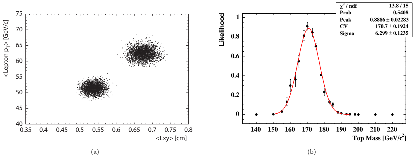
FIG. 10: (a): distribution of mean L_{xy} versus mean lepton p_T from pseudoexperiments for extreme mass cases of 140 GeV and 220 GeV. (b): the pseudoexperiment results for the 23 mass points considered are used to determine the likelihood of agreement with the data according to the metric of Equation 1, and the results are plotted and fitted here. The mean fit result is taken as the measurement result, and the RMS represents our statistical uncertainty.
