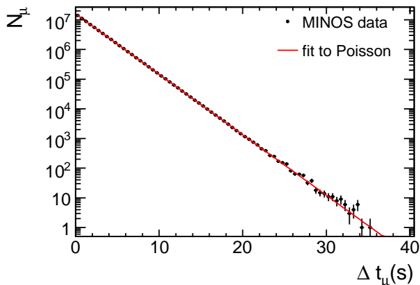
FIG. 2: The time between consecutive cosmic ray muon arrivals, fit with a Poisson distribution. The fit gives \chi^2/N_{Dof} = 55.2/68 ; \langle R_\mu \rangle = 0.4692 \pm 0.0001 Hz (from slope). The Poissonian nature of the muon arrival times demonstrates the absence of short timescale systematic effects on the data.
