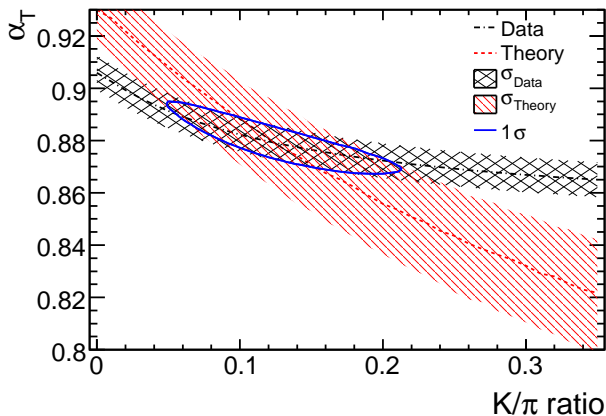
FIG. 7: The MINOS experimental \alpha_T as a function of the K/\pi ratio (dot-dash line), with its error given by the cross-hatched region, on the same axes as the theoretical \alpha_T as a function of the K/\pi ratio (dashed line), with its error given by the hatched region. The error on the experimental \alpha_T (from Table II E_{\text{th}} \cos \theta , B_{\pi,K}^1 and \langle T_{\text{eff}} \rangle ) plus statistical error is \pm 0.013 , and the theoretical \alpha_T error (from \epsilon_{\pi,K} and the rock map, Table III) is \pm 0.015 at the best fit point. The intersection is at K/\pi = 0.13 \pm 0.08 . The solid line denotes the 1\sigma contour around the best fit.
