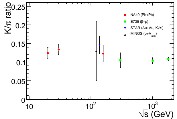
FIG. 8: A compilation of selected measurements of K/\pi for various center of mass energies. The STAR value was from Au+Au collisions at RHIC [28], the NA49 measurement was from Pb+Pb collisions at SPS [29, 30], and the E735 measurement was from \bar{p}+p collisions at the Tevatron [32].
