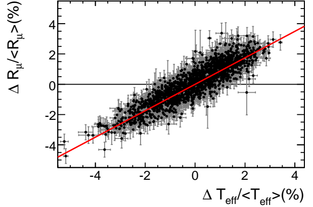
FIG. 5: A plot of \Delta R_\mu / \langle R_\mu \rangle as a function of \Delta T_{\text{eff}} / \langle T_{\text{eff}} \rangle for single muons, fit by a line with the y-intercept fixed at 0. The fit has a \chi^2/N_{Dof} = 1905/1797 , and the slope is \alpha_T = 0.874 \pm 0.009 .
