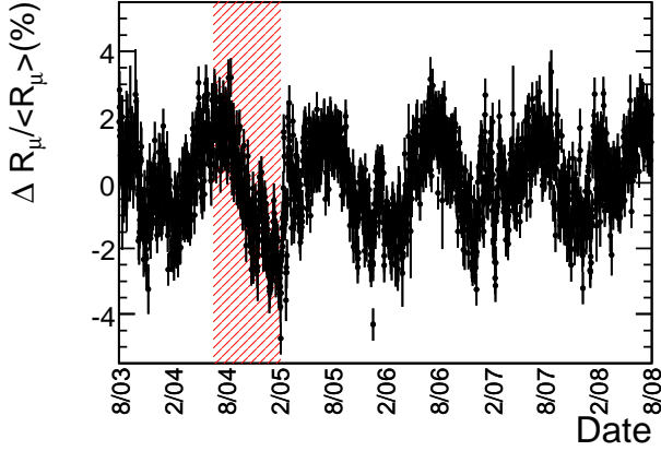
FIG. 3: The daily deviation from the mean rate of cosmic ray muon arrivals from 8/03-8/08, shown here with statistical error bars. The periodic fluctuations have the expected maxima in August, minima in February. The hatched region indicates the period of time when the detector ran with the magnetic field reversed from the normal configuration.
