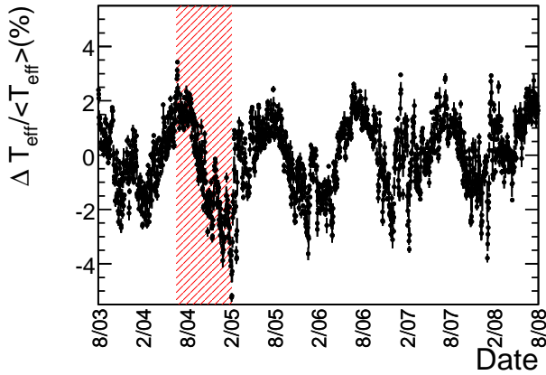
FIG. 4: The daily deviation from the mean effective temperature over a period of five years, beginning when the far detector was complete, 08/03-08/08. The hatched region indicates the period of time when the detector ran with the magnetic field reversed from the normal configuration.
