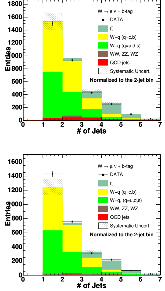
FIG. 7: The measured distributions (points) in the number of jets in events with a W and a b -tag for W \rightarrow e\nu and W \rightarrow \mu\nu , compared to SM expectations (histogram). The order of stacking in the histograms is the same as in their legends.
