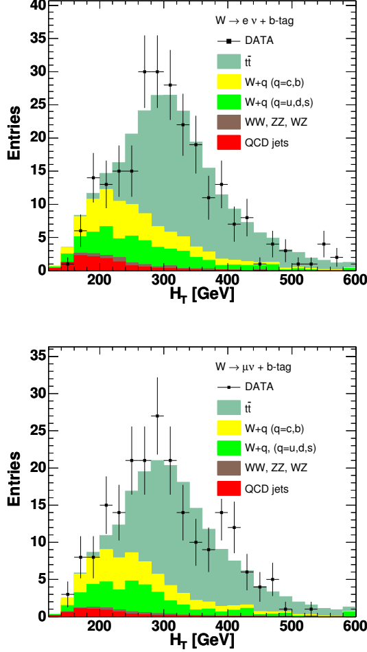
FIG. 8: The measured distribution (points) in H_T in events with a W and a b -tag, compared to SM expectations (histogram), for the electron channel (upper figure) and muon channel (lower figure). The order of stacking in the histograms is the same as in their legends.
