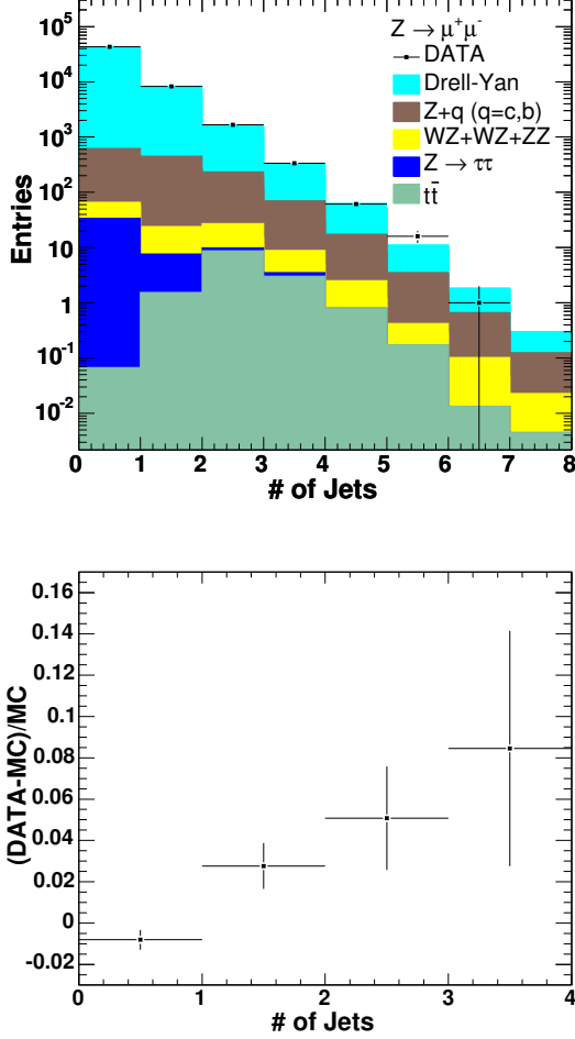
FIG. 11: The measured distribution (points) in the number of jets in events with an inclusive decay of Z \rightarrow \mu^+ \mu^- , compared to SM expectations (stacked histogram). The order of stacking in the histogram is the same as in the legend. The Z +jets processes (Drell-Yan, Z+b , and Z+c ) are modeled with ALPGEN. The lower plot shows the difference between the data and predictions.
