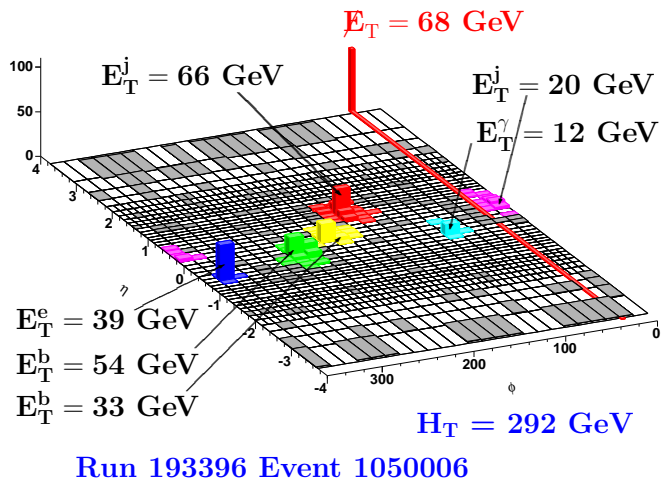
FIG. 5: The \eta - \phi plot of a t\bar{t}\gamma candidate event, in which the energies deposited in the calorimeter towers are displayed in the \eta - \phi plane. The reconstructed top quark mass is 167 GeV; the photon E_T is 12 GeV.
