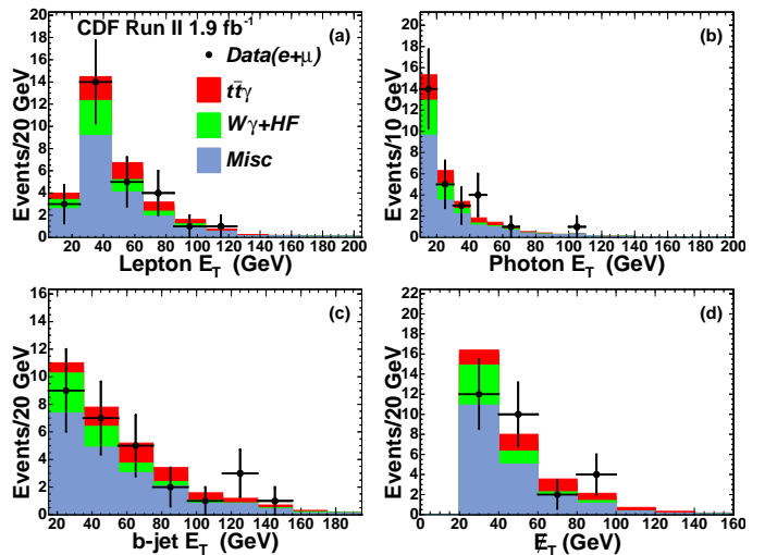
FIG. 1: The distributions for events in the \ell\gamma b\cancel{E}_T sample (points) in a) the E_T of the lepton; b) the E_T of the photon; c) the E_T of the most energetic b -jet in an event; and d) the missing transverse energy. The histograms show the estimated SM contributions from radiative top quark decay ( t\bar{t}\gamma ), WZ production, W\gamma production with heavy flavor (HF), \tau leptons, electrons, and jets misidentified as photons, mistagged light-quark and gluon jets, and jets misidentified as leptons (QCD).
