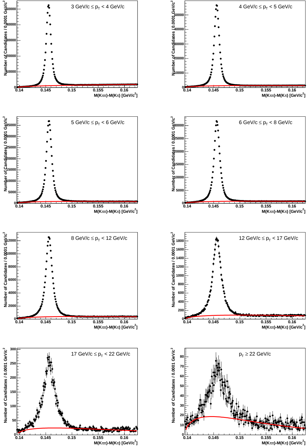
FIG. 5: The m(K\pi\pi) - m(K\pi) distribution for D^{*\pm} \rightarrow D^0\pi^\pm, D^0 \rightarrow K^\mp\pi^\pm candidates in different SLT \mu -track- P_T bins. The line in each plot represents the fit to the sideband regions.
