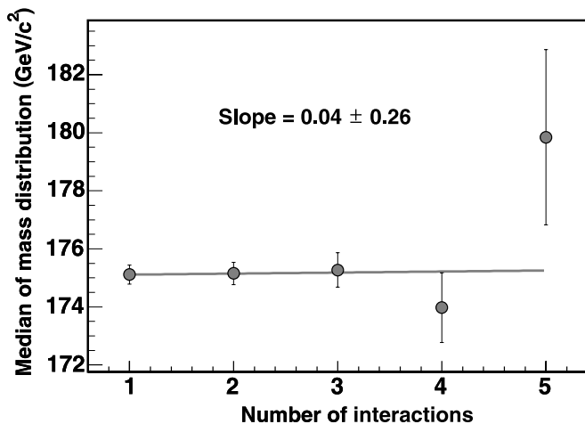
FIG. 10: Results from PE’s performed using events selected according to the number of interactions.
