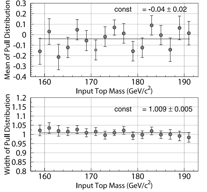
FIG. 7: Results from pseudo-experiments: mean and width of the pull distributions versus generated top quark mass are shown in the upper and lower plots respectively.
