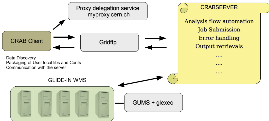
Figure 6. Schematic diagram of CRABserver in association with glideinWMS.
