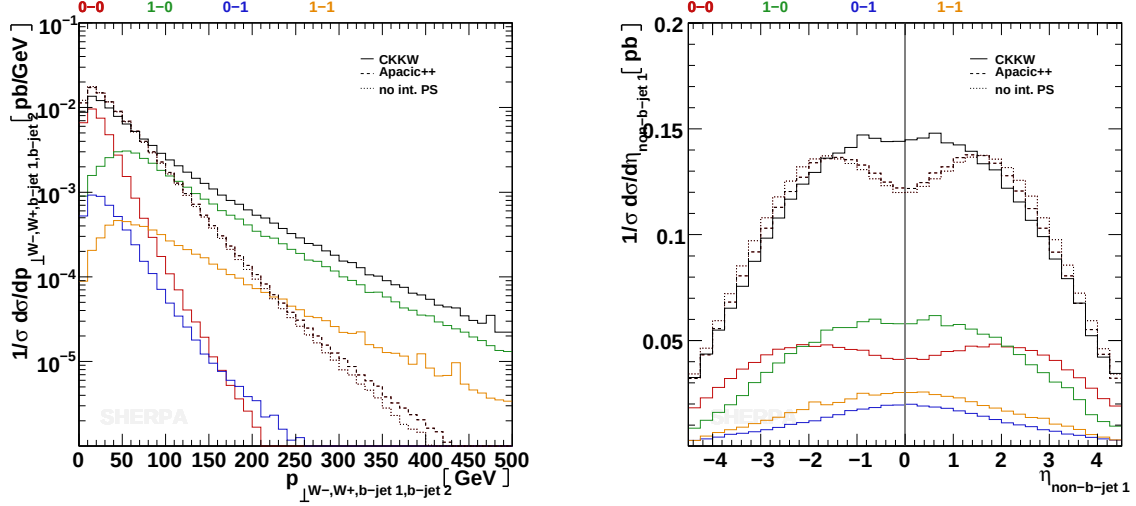
Fig. 14 Transverse momentum spectrum of the t\bar{t} -pair (left panel) and rapidity spectrum of the first extra jet (right panel) in pp \rightarrow t\bar{t} \rightarrow W^+W^-b\bar{b} + \text{jets} events at \sqrt{s} = 14 TeV. Shown is a comparison between the pure parton-shower result (no int. PS), parton shower with radiation off intermediate top quarks (Apacic++) and a CKKW-merged sample. Contributions from various matrix element configurations are highlighted in colour for the merged sample, with the colour code indicating the additional jet multiplicity in the production \otimes decay process. Up to one extra jet has been simulated through matrix elements in the production and each decay.
