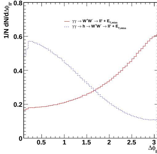
Fig. 5 Lepton azimuthal separation in \gamma\gamma \rightarrow W^+W^- \rightarrow \ell\ell' + \cancel{E}_T with and without an intermediate Standard Model Higgs boson of m_H = 160 GeV.
