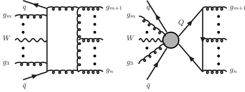
Figure 1: Parent diagrams for primitive amplitudes A_n^L(1_{\bar{q}}, 3_g, \dots, m_g, 2_q, m+1_g, \dots, n_g) and A_n^{L,[1/2]}(1_{\bar{q}}, 3_g, \dots, m_g, 2_q, (m+1)_g, \dots, n_g) . All other parent diagrams that contribute to this primitive are obtained by considering all possible insertions of the W boson without changing relative ordering of quarks and gluons. The shaded circle stands for dummy lines.
