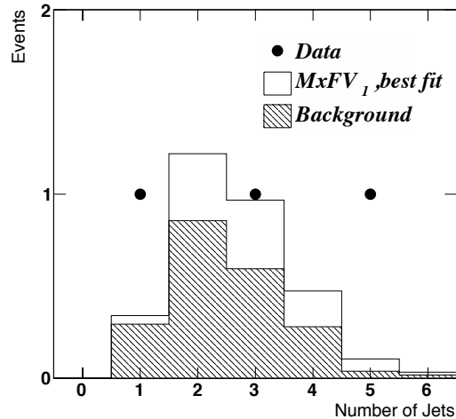
FIG. 2: Jet multiplicity for background, observed data, and MxFV_1 signal with best-fit value of \xi = 0.41 for M_{\eta^0} = 180 \text{ GeV}/c^2 .
