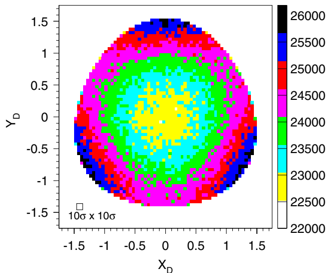
FIG. 5 (color online). Dalitz plot density, Y_D vs X_D , for 68.3 \times 10^6 K_L \rightarrow \pi^0\pi^0\pi^0 decays in the KTeV data sample after all selection requirements. The color scale at the right shows the number of events in each 0.05 \times 0.05 pixel. The reconstruction resolution on X_D and Y_D is \sigma \sim 0.01 as determined by the MC; the box in the lower-left corner shows 10\sigma \times 10\sigma for illustration.
