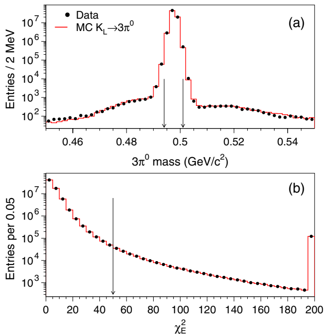
FIG. 4 (color online). (a) Invariant \pi^0\pi^0\pi^0 mass with all selection requirements except for the \pi^0\pi^0\pi^0 mass and \chi^2_E . The \pi^0\pi^0\pi^0 mass resolution (from Gaussian fit) is 0.94 \text{ MeV}/c^2 . (b) shows \chi^2_E distribution with all other selection requirements; last bin includes all events with \chi^2_E > 200 . Dots are data and the histogram is MC. Vertical arrows show the selection requirements.
