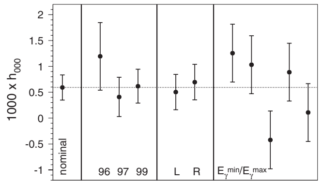
FIG. 7. Cross-check measurements of h_{000} : data-taking years (96,97,99), left and right vacuum beams (L,R), and min/max photon-energy ratio ( E_{\gamma}^{\min}/E_{\gamma}^{\max} ) as discussed in the text. Measurements within each category (between vertical lines) are statistically independent. Error bars reflect the statistical uncertainties from the data and MC samples.
