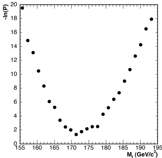
FIG. 3: Negative of the logarithm of the joint probability density as a function of top quark mass for the 344 candidate events after all corrections. Systematic uncertainties are not shown.
