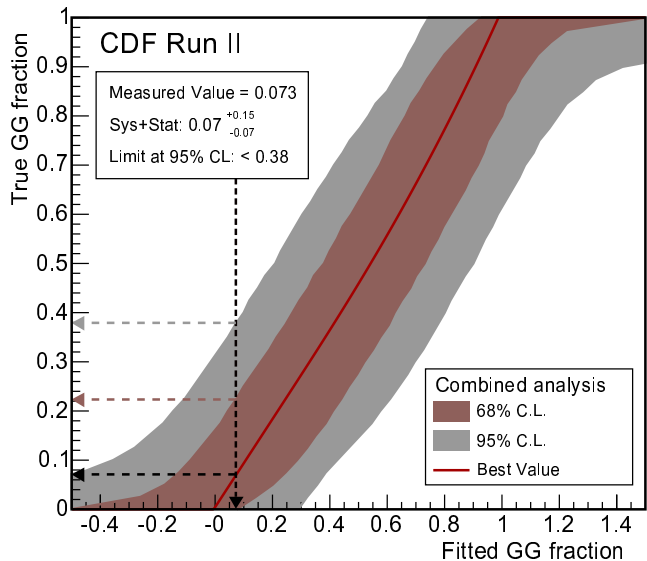
FIG. 2: Feldman-Cousins bands with statistical and systematic uncertainties for 68% C.L. and 95% C.L.. In the data, we find G_f^{fit} = 0.073 , which yields G_f = 0.07_{-0.07}^{+0.15} and G_f < 0.38 at the 95% C.L..
