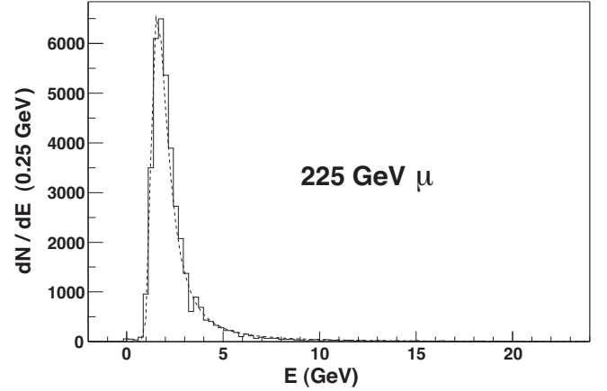
Fig. 16. Observed energy distribution in the HB for 225 GeV/c incident muons. The most probable value for the energy deposited is 1.64 GeV while the mean is 2.5 GeV. The dashed curve is the result of a fit by a Landau distribution.
