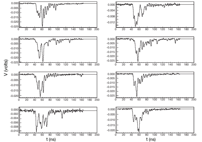
Fig. 10. Calorimeter pulses for eight individual events, voltage vs time, observed with a photomultiplier for 225 GeV/c incident muons.
