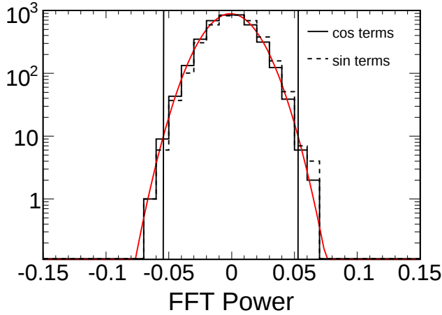
FIG. 2: The distributions for the even (cos) and the odd (sin) mean powers for harmonic frequencies to 4\omega_{\oplus}T_{\oplus} from the FFT analysis of 1,000 simulated experiments in Run I and Run II. Superposed on these distributions is a Gaussian fit of width \sigma = 1.8 \times 10^{-2} . This fit was obtained independently for both distributions. Values outside of the vertical lines are more than 3\sigma from the mean.
