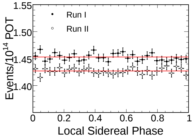
FIG. 1: The local sidereal phase histograms for Run I and Run II. Superposed are fits to a constant sidereal rate.
