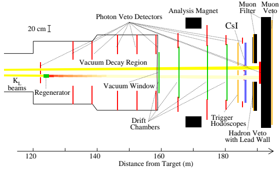
FIG. 1: Schematic of the KTeV detector.
