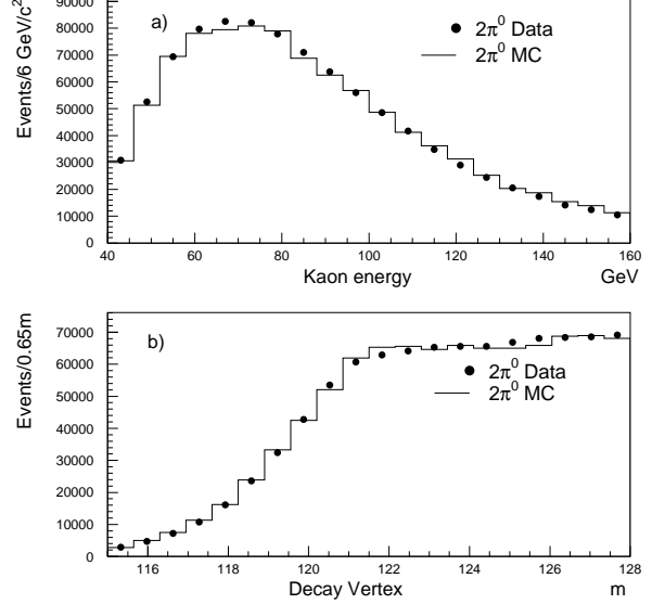
FIG. 7: The a) energy and b) decay vertex for K_L \rightarrow \pi^0 \pi^0 decays. The dots are the data and the histogram is the Monte Carlo simulation.
