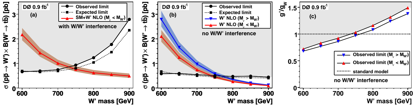
FIG. 2: NLO theory cross sections and 95% C.L. limits for \sigma_{W'} \times \text{B}(W' \rightarrow tb) as a function of W' mass for (a) W'_L production and (b) W'_R production. Observed limits on the ratio of coupling constants g'/g_w are shown in (c). The shaded regions are excluded by this analysis.
