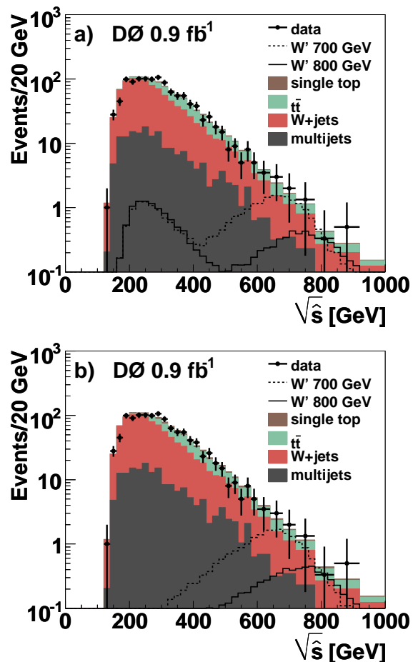
FIG. 1: \sqrt{\hat{s}} distributions for the data and the SM background. Plot (a) shows the W'_L signal and plot (b) shows the W'_R signal at two different masses, normalized to the NLO prediction (Table II). Events in the eight subsamples (electron, muon, two and three jets, single-tagged and double-tagged) are combined.
