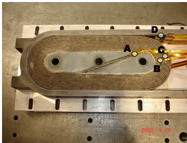
Fig. 1. The coil of the SR07 magnet is shown here after its heat treatment and just before epoxy impregnation. The central connecting cable is shown in the central iron pole just after rising from the bottom coil up to the top coil. The locations of the central voltage tap A and the intermediate voltage taps B and C, and the voltage tap at the splice D for the top coil are indicated.
